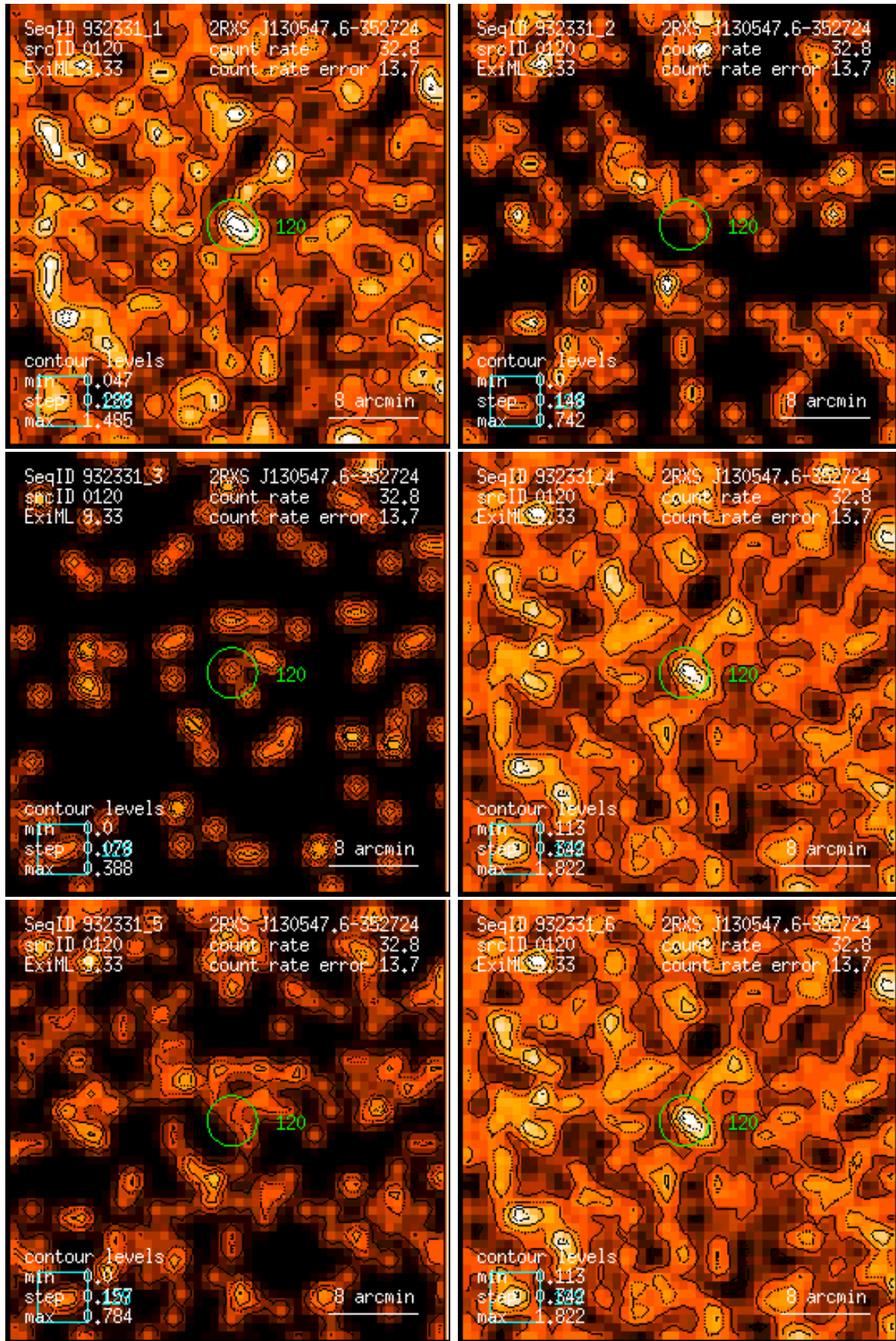
Figure 120: RASS 932331: detection 0120: band rate images, Gaussian filter: (1) PSPC channels 11 – 41, (2) 52 – 90, (3) 91 – 201, (4) 11 – 235, (5) 52 – 201, (6) 11 – 201. Broad band rates in counts/ks. Band rate contour levels in counts/ks/arcmin 2 .
