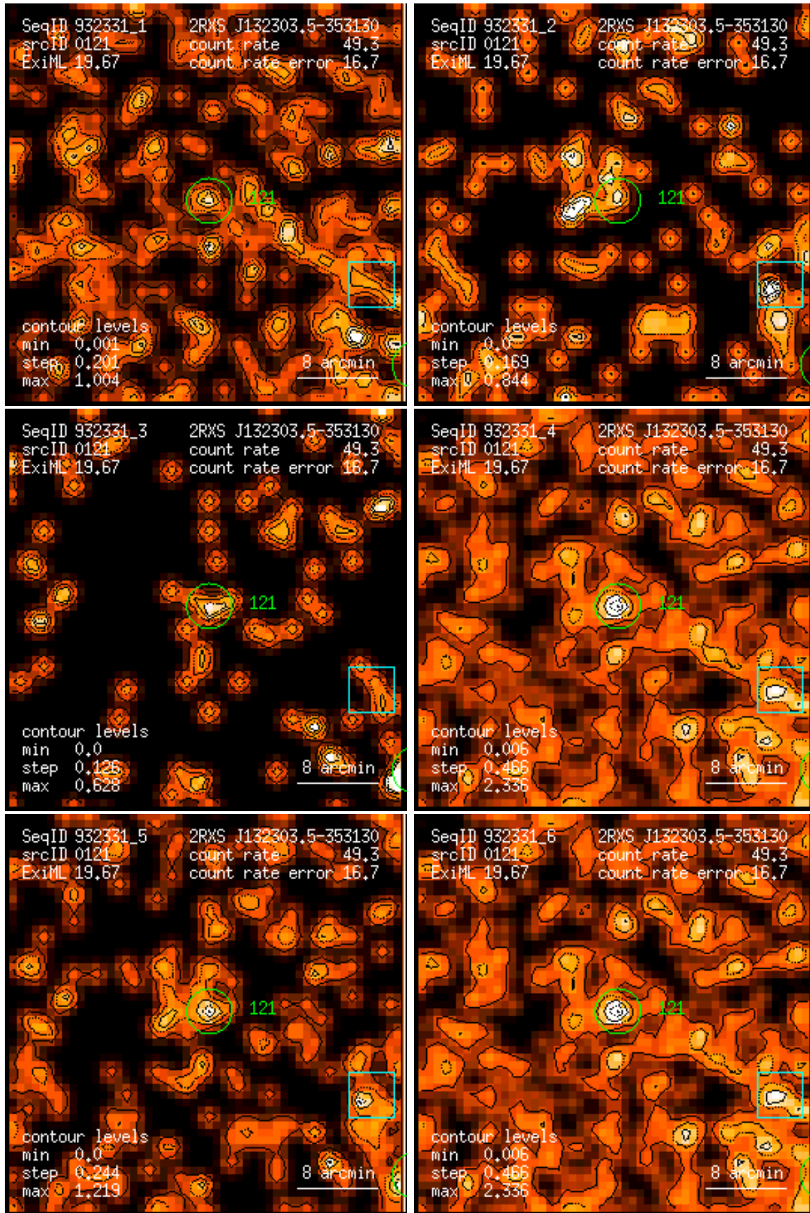
Figure 121: RASS 932331: detection 0121: band rate images, Gaussian filter: (1) PSPC channels 11 – 41, (2) 52 – 90, (3) 91 – 201, (4) 11 – 235, (5) 52 – 201, (6) 11 – 201. Broad band rates in counts/ks. Band rate contour levels in counts/ks/arcmin 2 .
