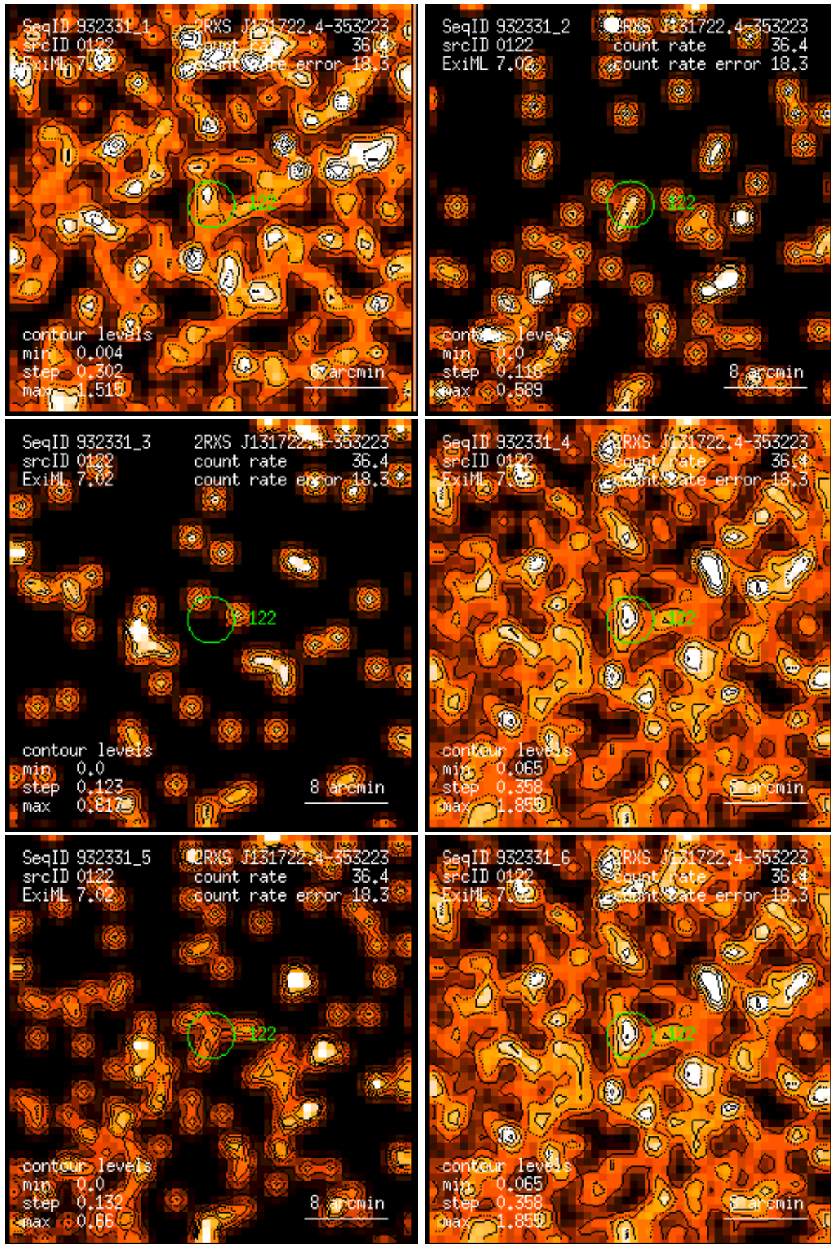
Figure 122: RASS 932331: detection 0122: band rate images, Gaussian filter: (1) PSPC channels 11 – 41, (2) 52 – 90, (3) 91 – 201, (4) 11 – 235, (5) 52 – 201, (6) 11 – 201. Broad band rates in counts/ks. Band rate contour levels in counts/ks/arcmin 2 .
