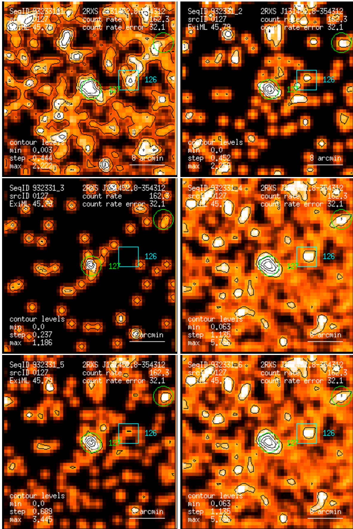
Figure 127: RASS 932331: detection 0127: band rate images, Gaussian filter: (1) PSPC channels 11 – 41, (2) 52 – 90, (3) 91 – 201, (4) 11 – 235, (5) 52 – 201, (6) 11 – 201. Broad band rates in counts/ks. Band rate contour levels in counts/ks/arcmin 2 .
