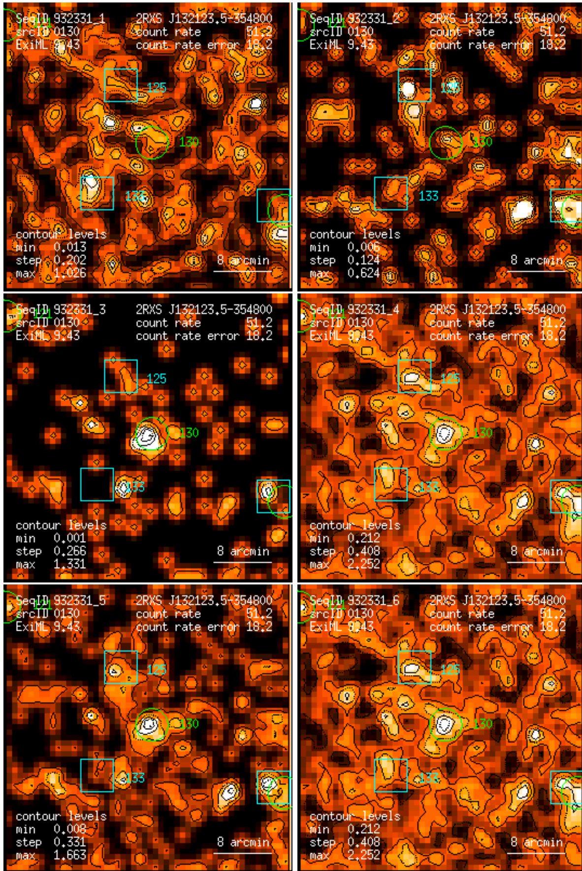
Figure 130: RASS 932331: detection 0130: band rate images, Gaussian filter: (1) PSPC channels 11 – 41, (2) 52 – 90, (3) 91 – 201, (4) 11 – 235, (5) 52 – 201, (6) 11 – 201. Broad band rates in counts/ks. Band rate contour levels in counts/ks/arcmin 2 .
