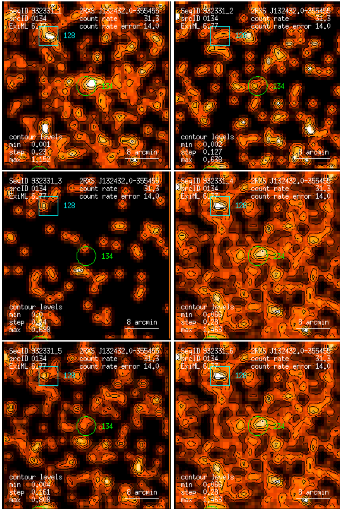
Figure 134: RASS 932331: detection 0134: band rate images, Gaussian filter: (1) PSPC channels 11 – 41, (2) 52 – 90, (3) 91 – 201, (4) 11 – 235, (5) 52 – 201, (6) 11 – 201. Broad band rates in counts/ks. Band rate contour levels in counts/ks/arcmin 2 .
