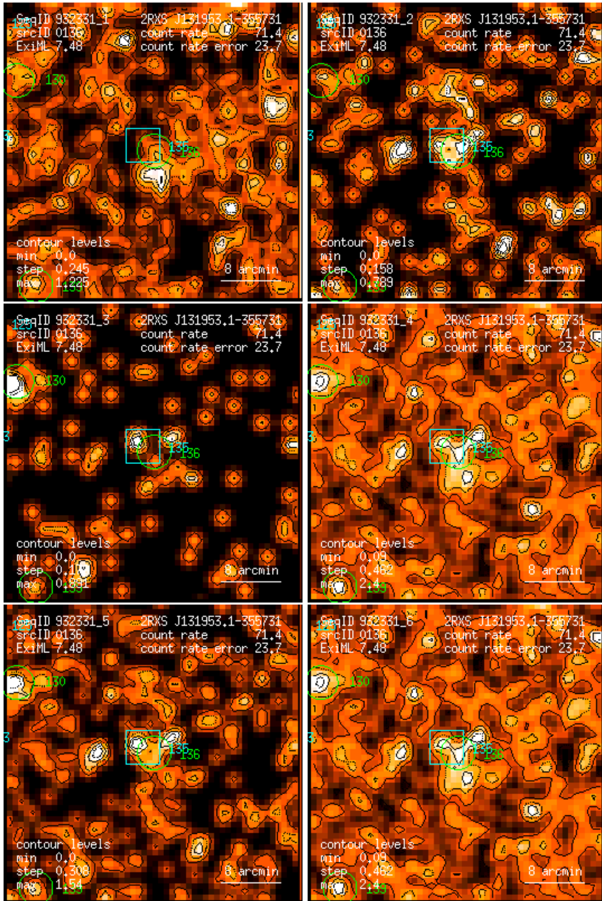
Figure 136: RASS 932331: detection 0136: band rate images, Gaussian filter: (1) PSPC channels 11 – 41, (2) 52 – 90, (3) 91 – 201, (4) 11 – 235, (5) 52 – 201, (6) 11 – 201. Broad band rates in counts/ks. Band rate contour levels in counts/ks/arcmin 2 .
