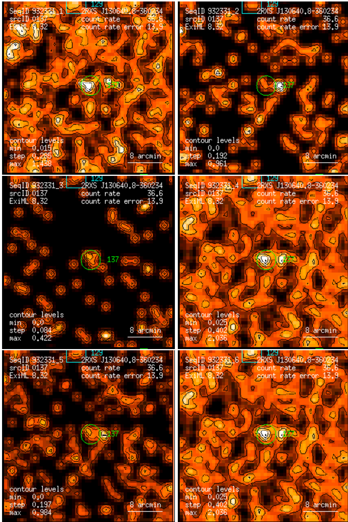
Figure 137: RASS 932331: detection 0137: band rate images, Gaussian filter: (1) PSPC channels 11 – 41, (2) 52 – 90, (3) 91 – 201, (4) 11 – 235, (5) 52 – 201, (6) 11 – 201. Broad band rates in counts/ks. Band rate contour levels in counts/ks/arcmin 2 .
