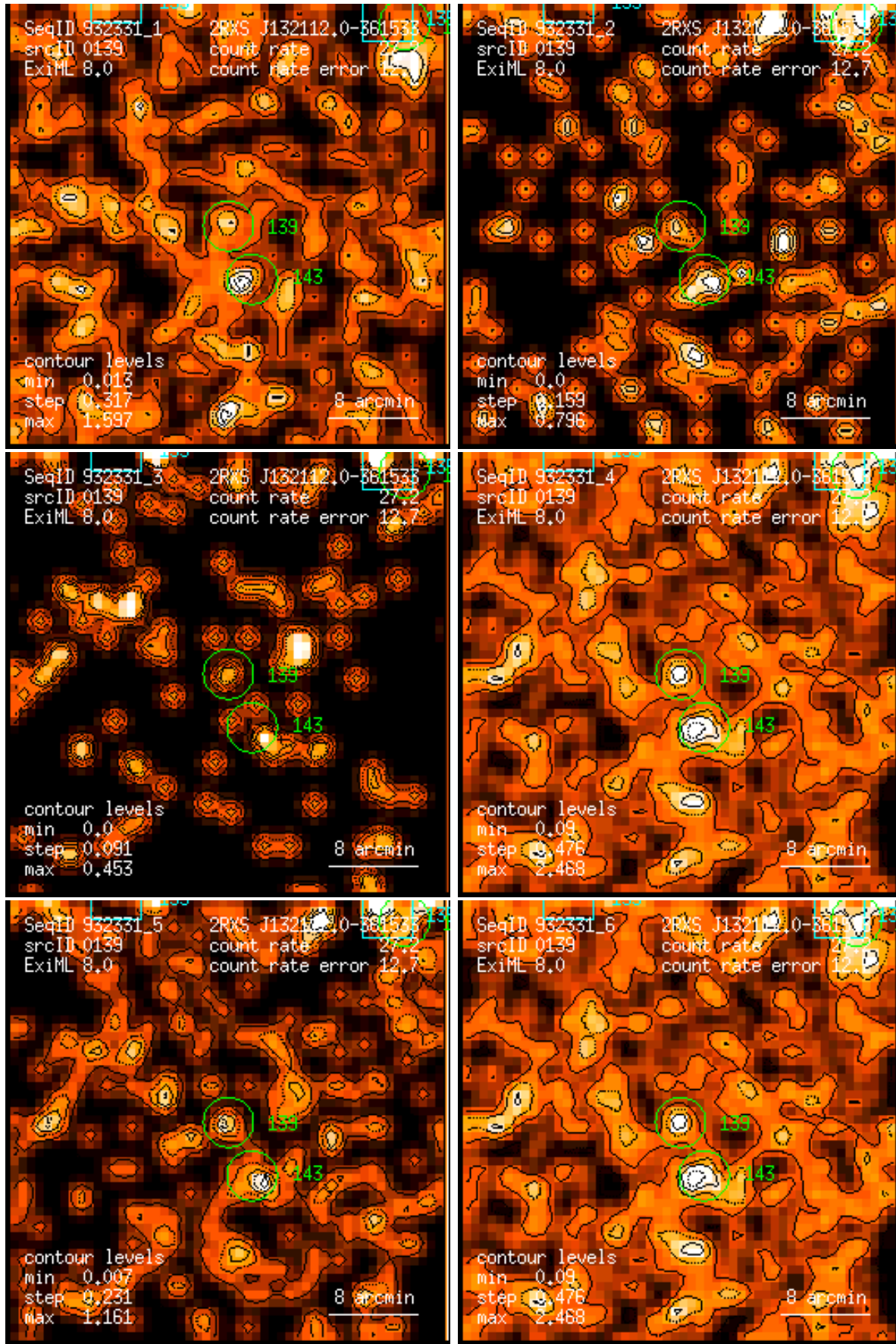
Figure 139: RASS 932331: detection 0139: band rate images, Gaussian filter: (1) PSPC channels 11 – 41, (2) 52 – 90, (3) 91 – 201, (4) 11 – 235, (5) 52 – 201, (6) 11 – 201. Broad band rates in counts/ks. Band rate contour levels in counts/ks/arcmin 2 .
