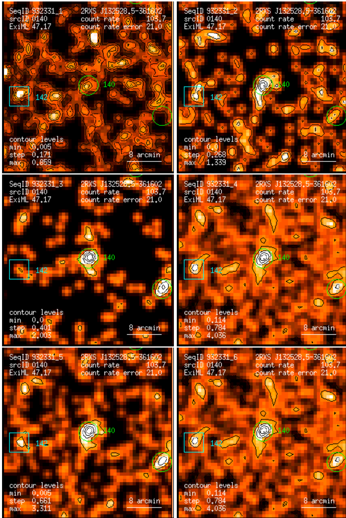
Figure 140: RASS 932331: detection 0140: band rate images, Gaussian filter: (1) PSPC channels 11 – 41, (2) 52 – 90, (3) 91 – 201, (4) 11 – 235, (5) 52 – 201, (6) 11 – 201. Broad band rates in counts/ks. Band rate contour levels in counts/ks/arcmin 2 .
