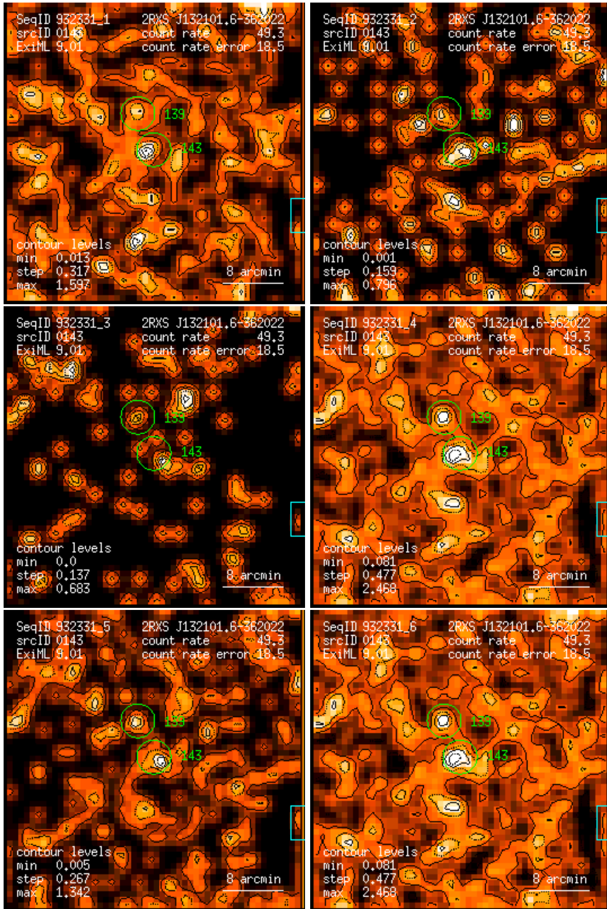
Figure 143: RASS 932331: detection 0143: band rate images, Gaussian filter: (1) PSPC channels 11 – 41, (2) 52 – 90, (3) 91 – 201, (4) 11 – 235, (5) 52 – 201, (6) 11 – 201. Broad band rates in counts/ks. Band rate contour levels in counts/ks/arcmin 2 .
