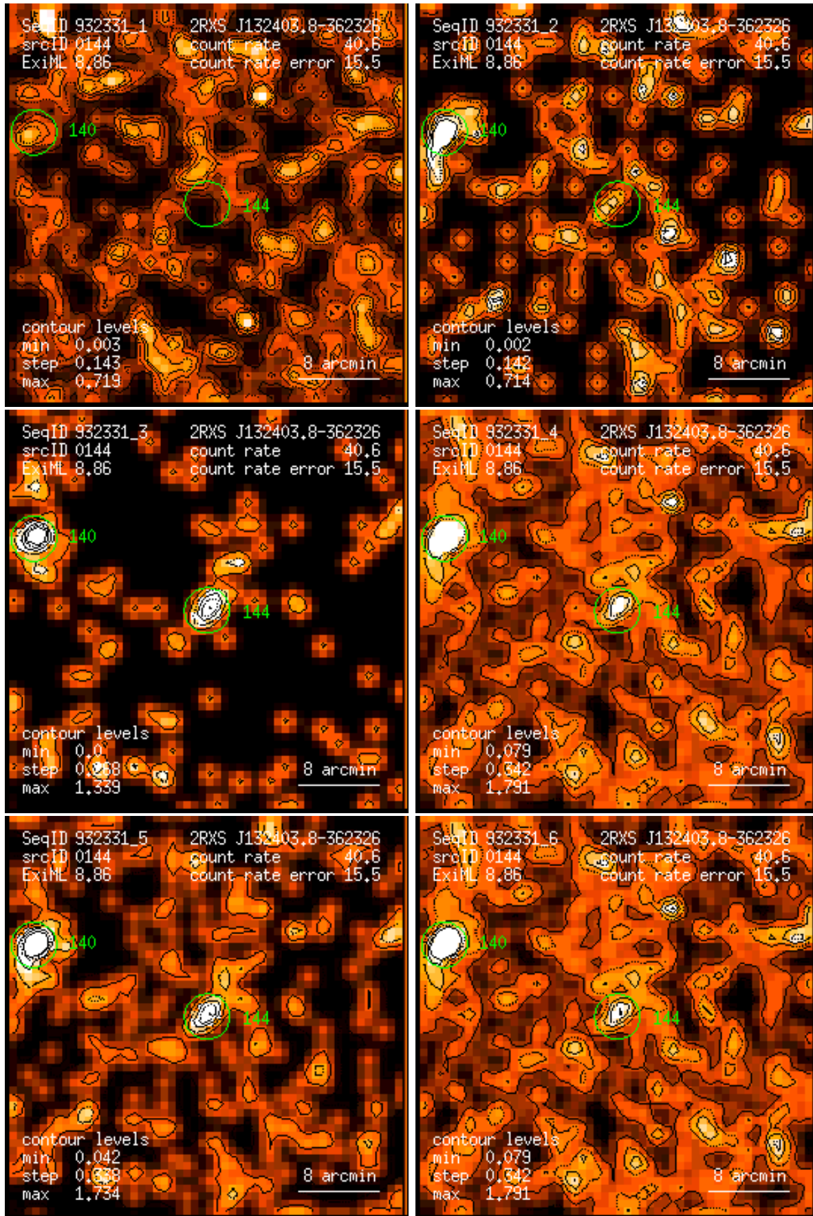
Figure 144: RASS 932331: detection 0144: band rate images, Gaussian filter: (1) PSPC channels 11 – 41, (2) 52 – 90, (3) 91 – 201, (4) 11 – 235, (5) 52 – 201, (6) 11 – 201. Broad band rates in counts/ks. Band rate contour levels in counts/ks/arcmin 2 .
