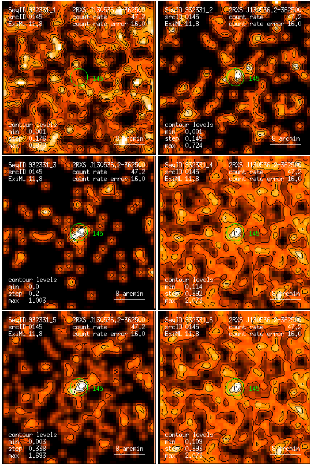
Figure 145: RASS 932331: detection 0145: band rate images, Gaussian filter: (1) PSPC channels 11 – 41, (2) 52 – 90, (3) 91 – 201, (4) 11 – 235, (5) 52 – 201, (6) 11 – 201. Broad band rates in counts/ks. Band rate contour levels in counts/ks/arcmin 2 .
