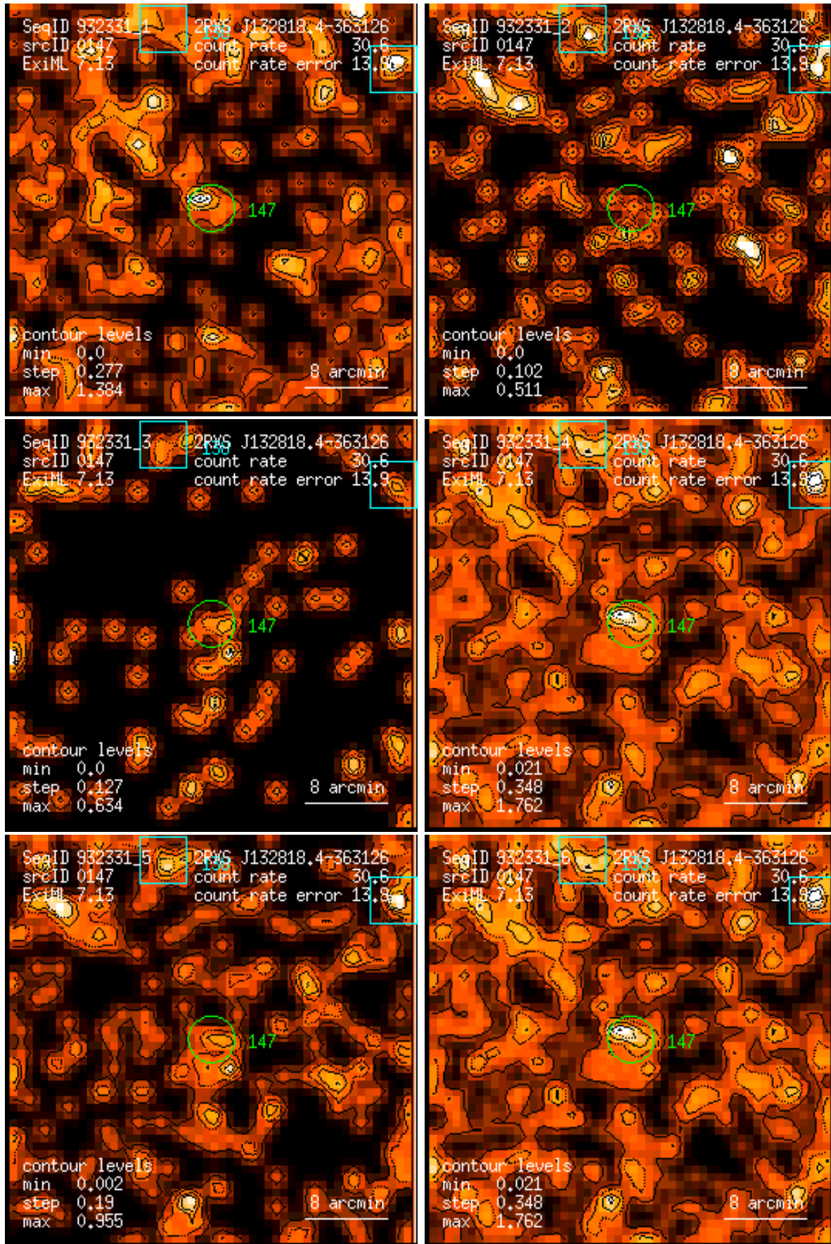
Figure 147: RASS 932331: detection 0147: band rate images, Gaussian filter: (1) PSPC channels 11 – 41, (2) 52 – 90, (3) 91 – 201, (4) 11 – 235, (5) 52 – 201, (6) 11 – 201. Broad band rates in counts/ks. Band rate contour levels in counts/ks/arcmin 2 .
