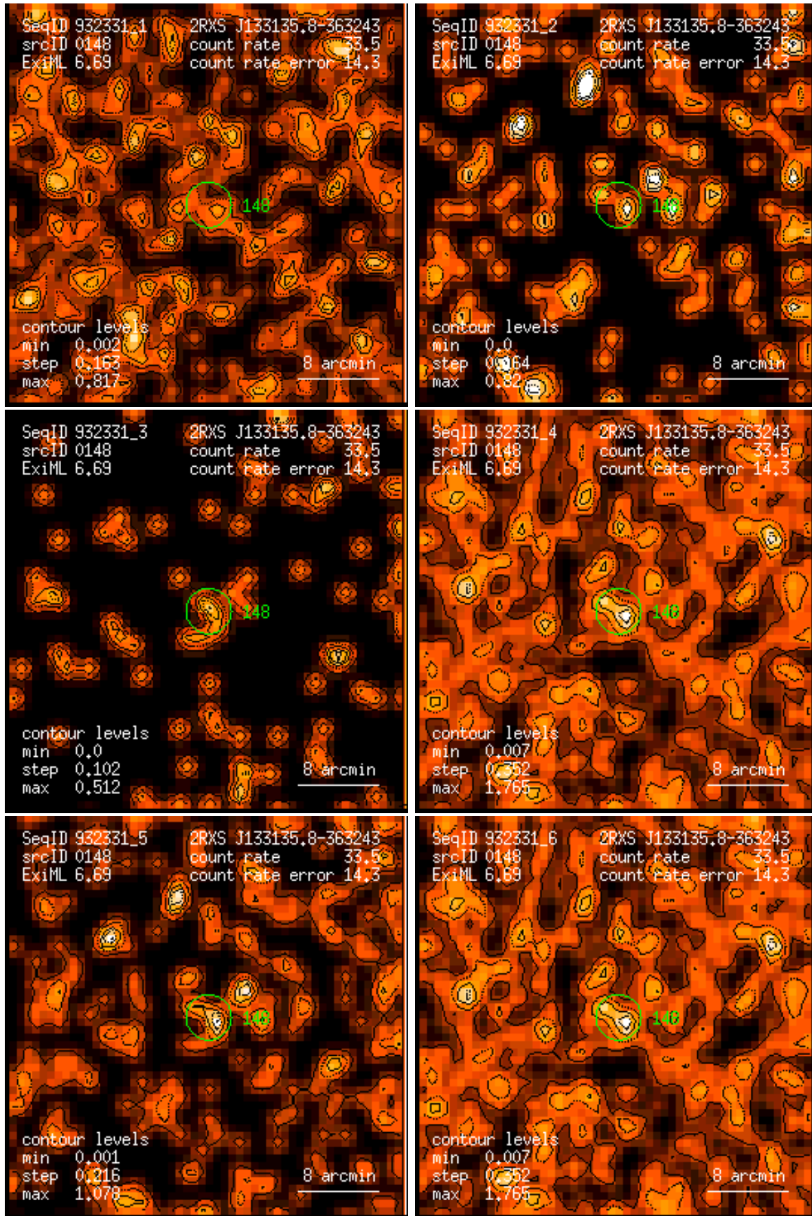
Figure 148: RASS 932331: detection 0148: band rate images, Gaussian filter: (1) PSPC channels 11 – 41, (2) 52 – 90, (3) 91 – 201, (4) 11 – 235, (5) 52 – 201, (6) 11 – 201. Broad band rates in counts/ks. Band rate contour levels in counts/ks/arcmin 2 .
