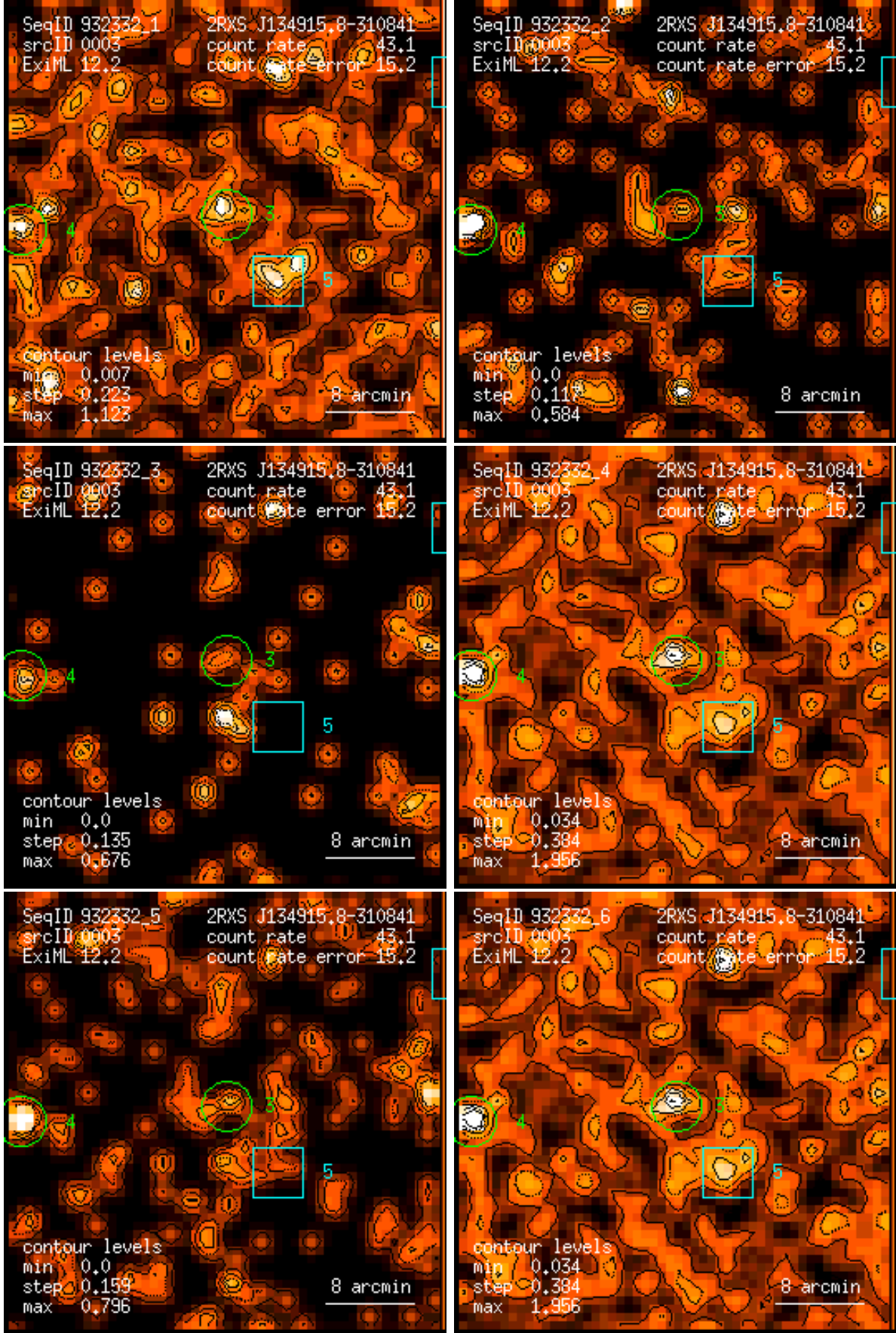
Figure 3: RASS 932332: detection 0003: band rate images, Gaussian filter: (1) PSPC channels 11 – 41, (2) 52 – 90, (3) 91 – 201, (4) 11 – 235, (5) 52 – 201, (6) 11 – 201. Broad band rates in counts/ks. Band rate contour levels in counts/ks/arcmin 2 .
