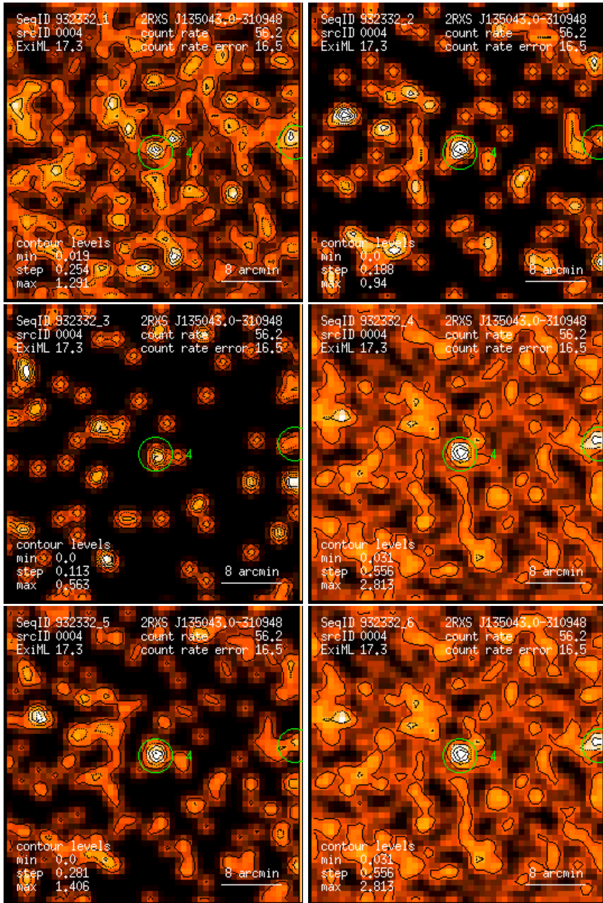
Figure 4: RASS 932332: detection 0004: band rate images, Gaussian filter: (1) PSPC channels 11 – 41, (2) 52 – 90, (3) 91 – 201, (4) 11 – 235, (5) 52 – 201, (6) 11 – 201. Broad band rates in counts/ks. Band rate contour levels in counts/ks/arcmin 2 .
