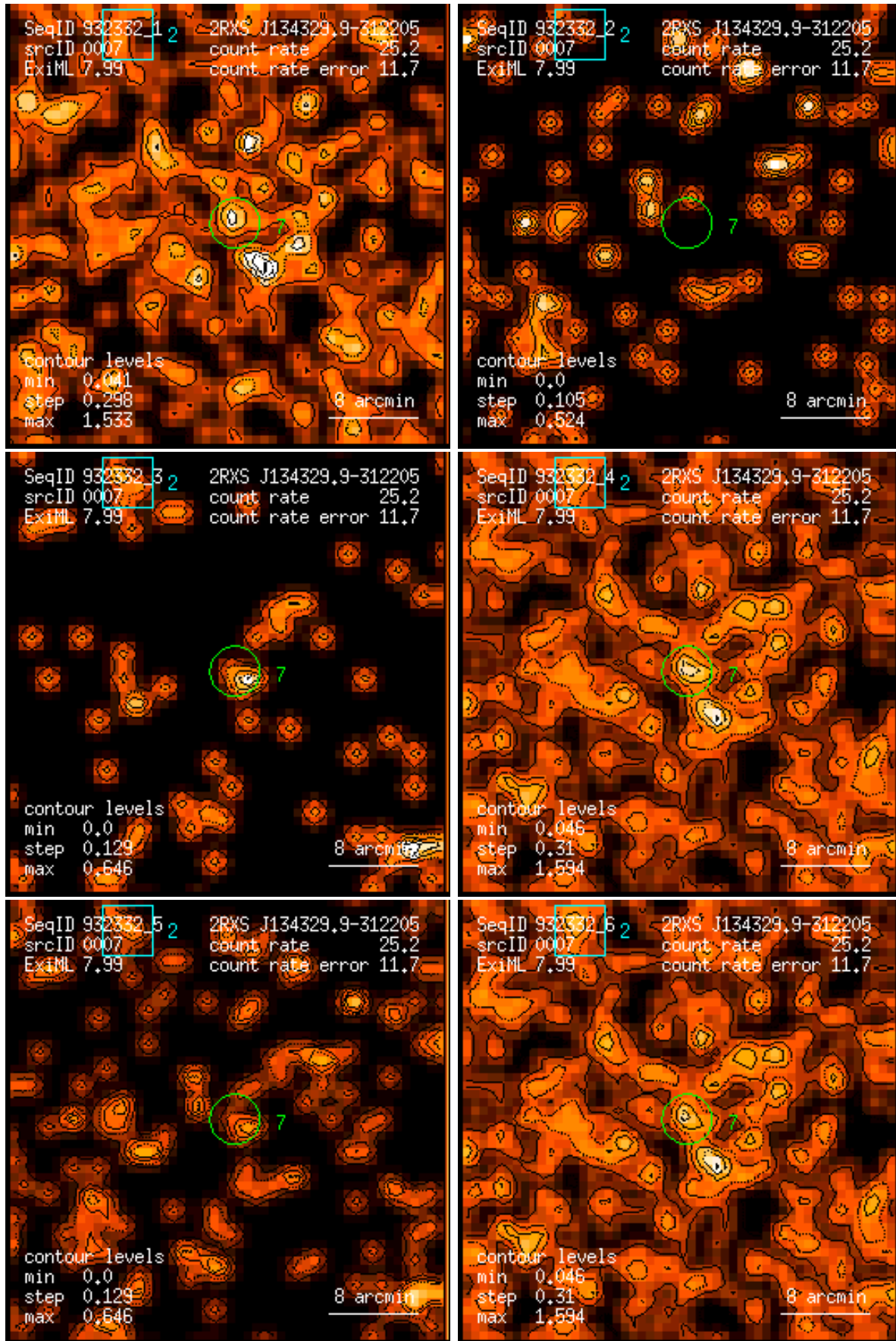
Figure 7: RASS 932332: detection 0007: band rate images, Gaussian filter: (1) PSPC channels 11 – 41, (2) 52 – 90, (3) 91 – 201, (4) 11 – 235, (5) 52 – 201, (6) 11 – 201. Broad band rates in counts/ks. Band rate contour levels in counts/ks/arcmin 2 .
