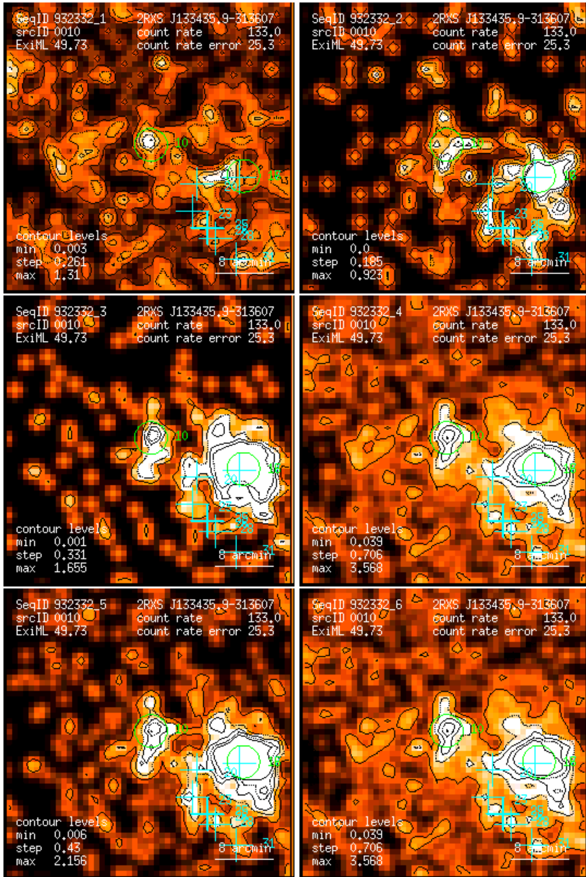
Figure 10: RASS 932332: detection 0010: band rate images, Gaussian filter: (1) PSPC channels 11 – 41, (2) 52 – 90, (3) 91 – 201, (4) 11 – 235, (5) 52 – 201, (6) 11 – 201. Broad band rates in counts/ks. Band rate contour levels in counts/ks/arcmin 2 .
