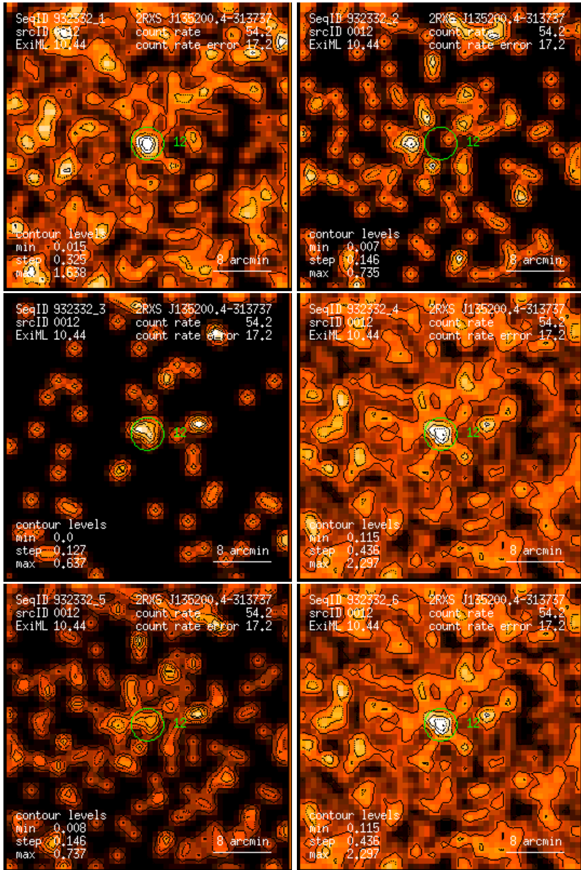
Figure 12: RASS 932332: detection 0012: band rate images, Gaussian filter: (1) PSPC channels 11 – 41, (2) 52 – 90, (3) 91 – 201, (4) 11 – 235, (5) 52 – 201, (6) 11 – 201. Broad band rates in counts/ks. Band rate contour levels in counts/ks/arcmin 2 .
