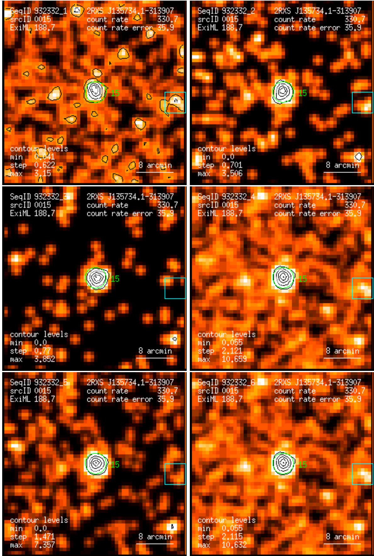
Figure 15: RASS 932332: detection 0015: band rate images, Gaussian filter: (1) PSPC channels 11 – 41, (2) 52 – 90, (3) 91 – 201, (4) 11 – 235, (5) 52 – 201, (6) 11 – 201. Broad band rates in counts/ks. Band rate contour levels in counts/ks/arcmin 2 .
