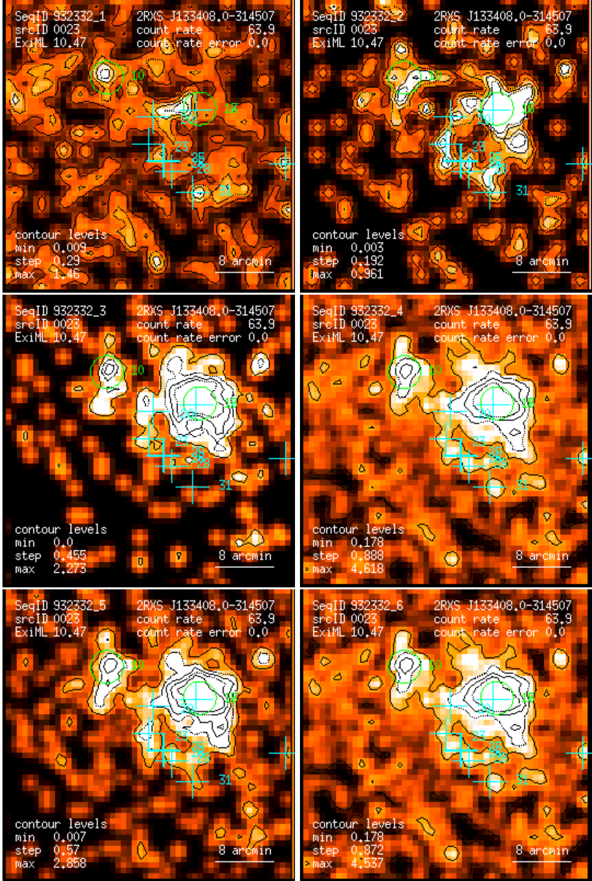
Figure 23: RASS 932332: detection 0023: band rate images, Gaussian filter: (1) PSPC channels 11 – 41, (2) 52 – 90, (3) 91 – 201, (4) 11 – 235, (5) 52 – 201, (6) 11 – 201. Broad band rates in counts/ks. Band rate contour levels in counts/ks/arcmin 2 .
