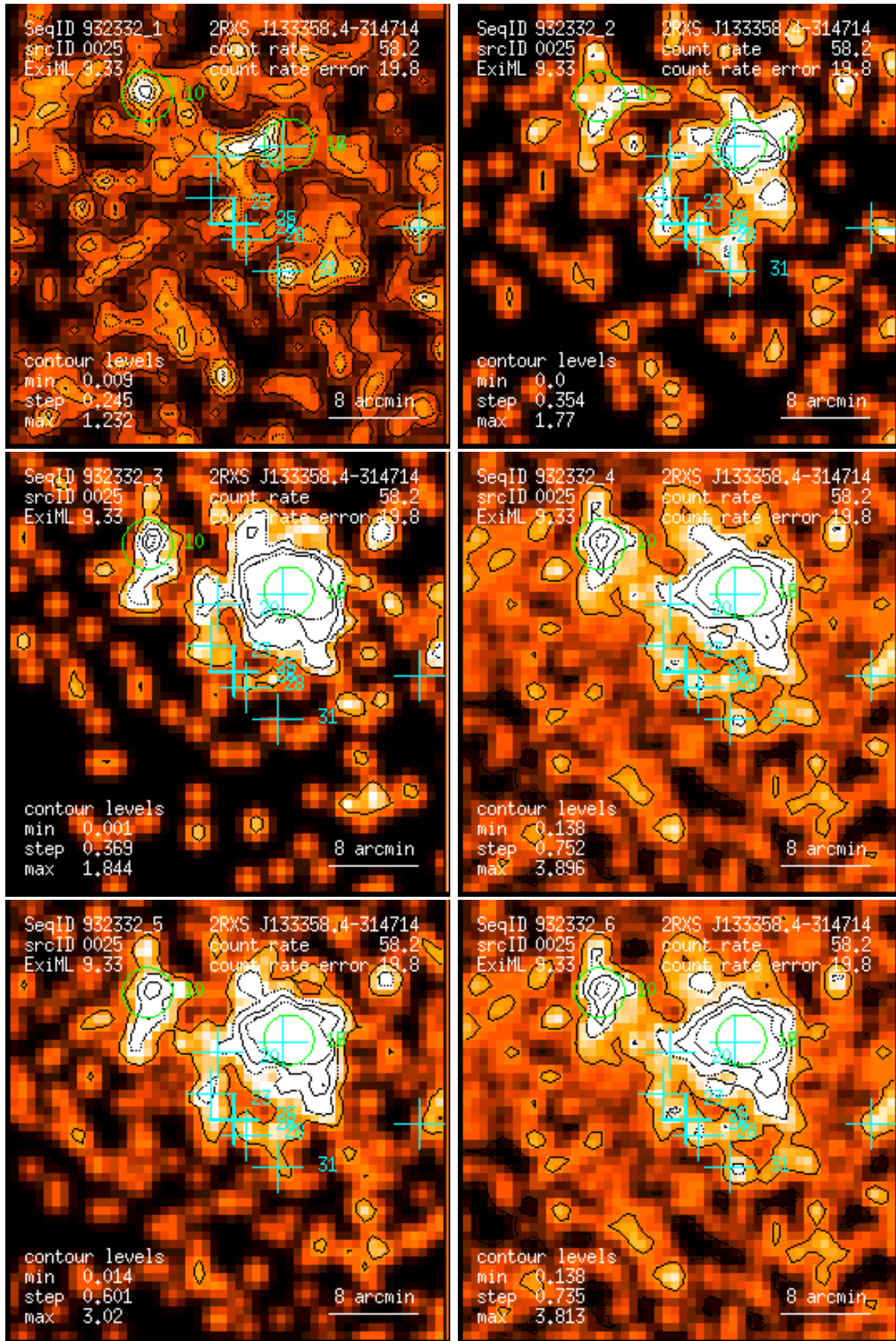
Figure 25: RASS 932332: detection 0025: band rate images, Gaussian filter: (1) PSPC channels 11 – 41, (2) 52 – 90, (3) 91 – 201, (4) 11 – 235, (5) 52 – 201, (6) 11 – 201. Broad band rates in counts/ks. Band rate contour levels in counts/ks/arcmin 2 .
