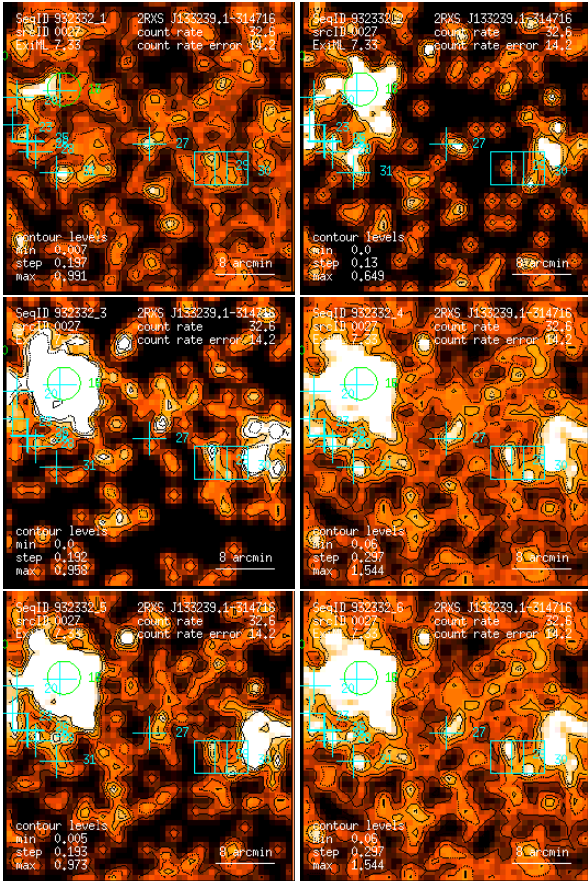
Figure 27: RASS 932332: detection 0027: band rate images, Gaussian filter: (1) PSPC channels 11 – 41, (2) 52 – 90, (3) 91 – 201, (4) 11 – 235, (5) 52 – 201, (6) 11 – 201. Broad band rates in counts/ks. Band rate contour levels in counts/ks/arcmin 2 .
