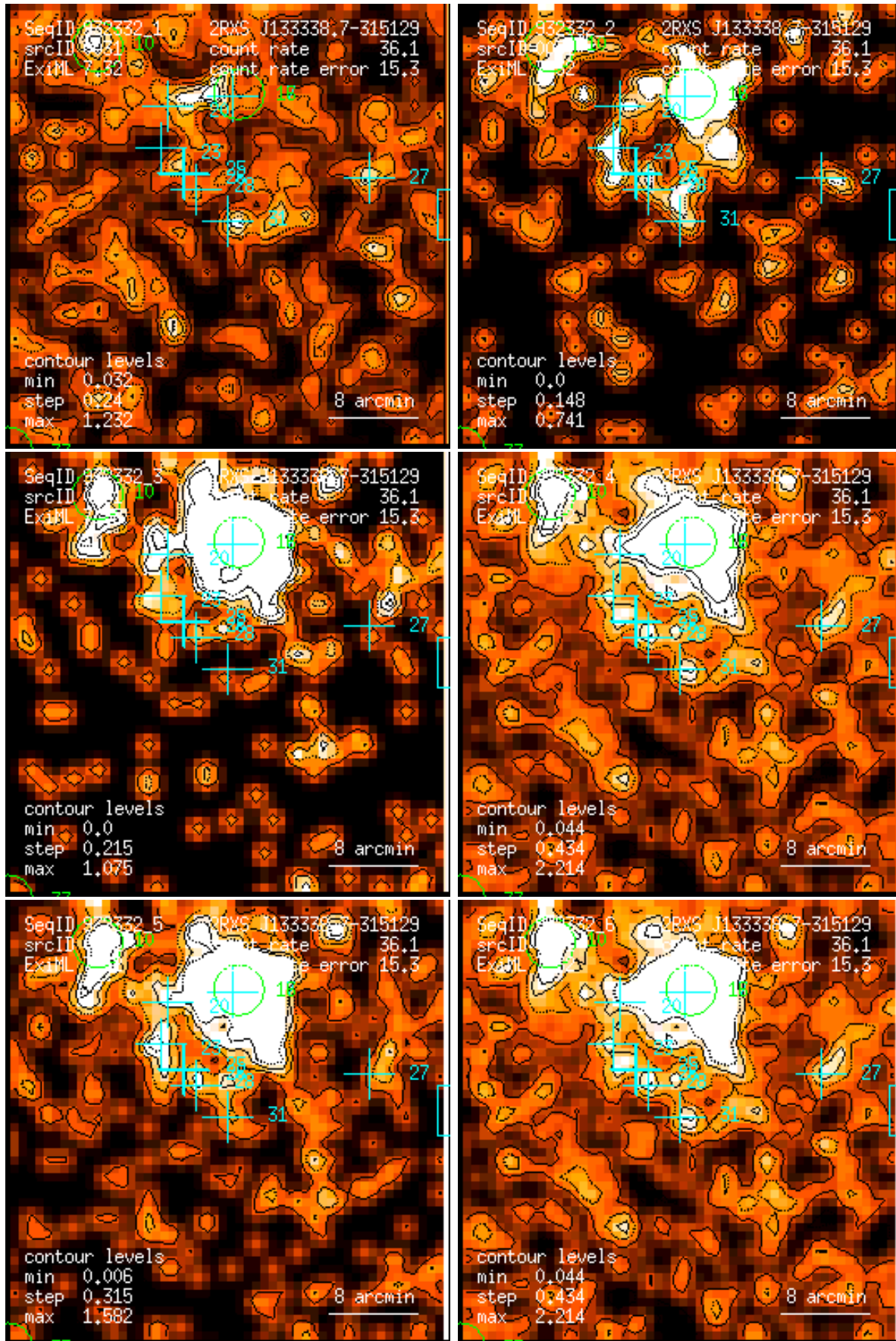
Figure 31: RASS 932332: detection 0031: band rate images, Gaussian filter: (1) PSPC channels 11 – 41, (2) 52 – 90, (3) 91 – 201, (4) 11 – 235, (5) 52 – 201, (6) 11 – 201. Broad band rates in counts/ks. Band rate contour levels in counts/ks/arcmin 2 .
