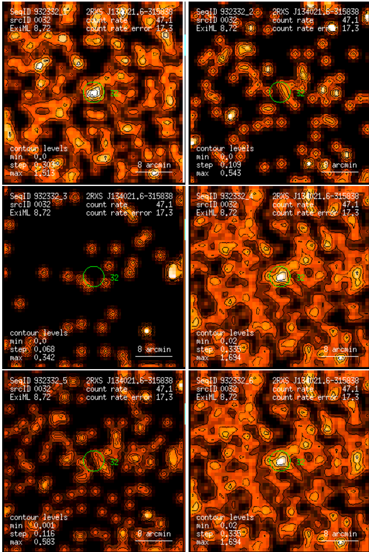
Figure 32: RASS 932332: detection 0032: band rate images, Gaussian filter: (1) PSPC channels 11 – 41, (2) 52 – 90, (3) 91 – 201, (4) 11 – 235, (5) 52 – 201, (6) 11 – 201. Broad band rates in counts/ks. Band rate contour levels in counts/ks/arcmin 2 .
