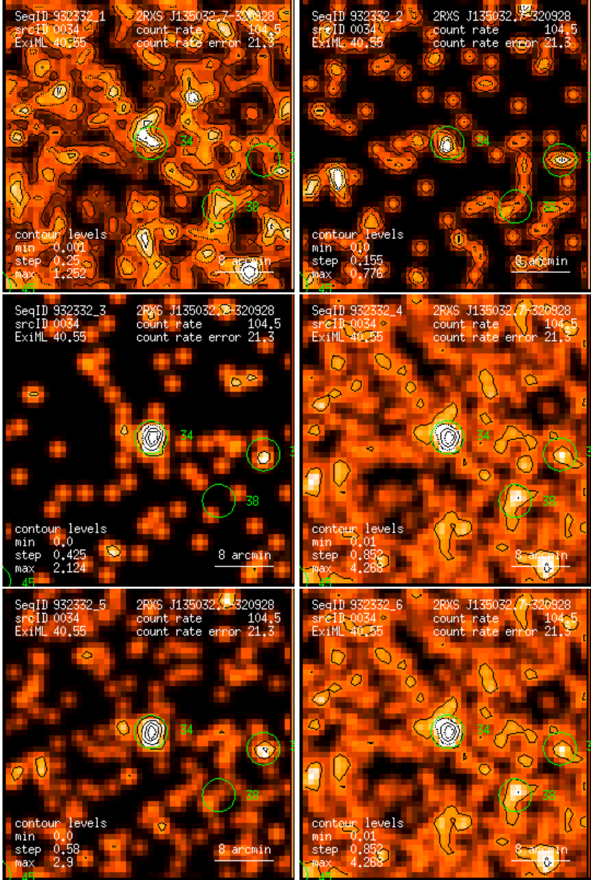
Figure 34: RASS 932332: detection 0034: band rate images, Gaussian filter: (1) PSPC channels 11 – 41, (2) 52 – 90, (3) 91 – 201, (4) 11 – 235, (5) 52 – 201, (6) 11 – 201. Broad band rates in counts/ks. Band rate contour levels in counts/ks/arcmin 2 .
