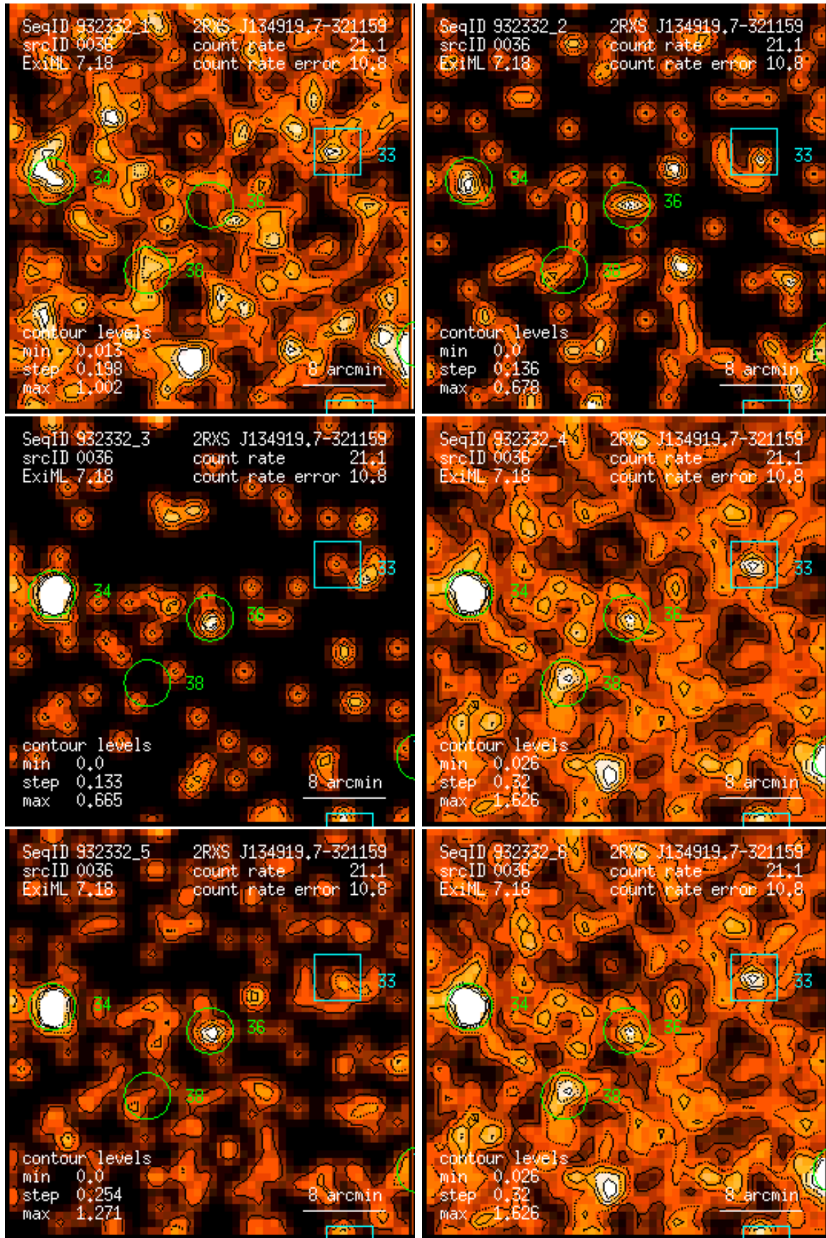
Figure 36: RASS 932332: detection 0036: band rate images, Gaussian filter: (1) PSPC channels 11 – 41, (2) 52 – 90, (3) 91 – 201, (4) 11 – 235, (5) 52 – 201, (6) 11 – 201. Broad band rates in counts/ks. Band rate contour levels in counts/ks/arcmin 2 .
