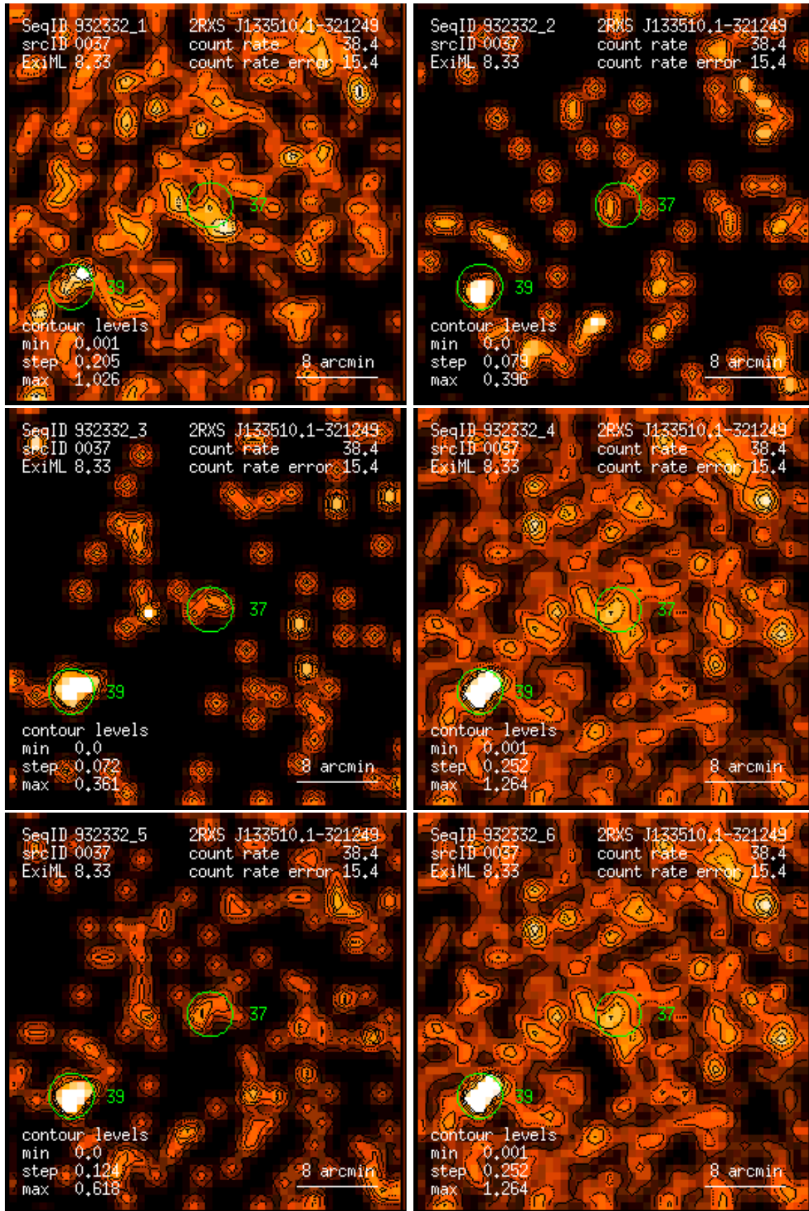
Figure 37: RASS 932332: detection 0037: band rate images, Gaussian filter: (1) PSPC channels 11 – 41, (2) 52 – 90, (3) 91 – 201, (4) 11 – 235, (5) 52 – 201, (6) 11 – 201. Broad band rates in counts/ks. Band rate contour levels in counts/ks/arcmin 2 .
