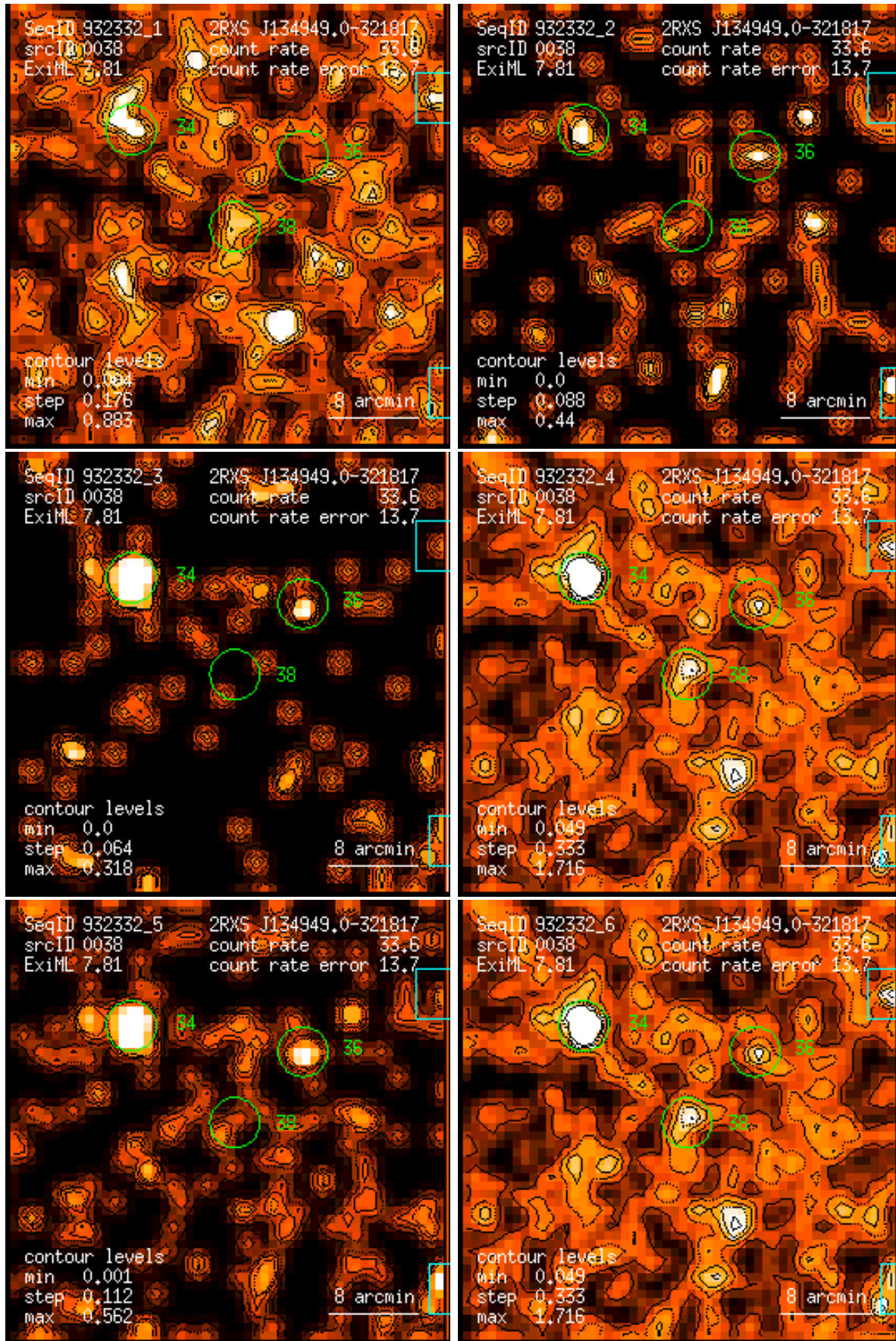
Figure 38: RASS 932332: detection 0038: band rate images, Gaussian filter: (1) PSPC channels 11 – 41, (2) 52 – 90, (3) 91 – 201, (4) 11 – 235, (5) 52 – 201, (6) 11 – 201. Broad band rates in counts/ks. Band rate contour levels in counts/ks/arcmin 2 .
