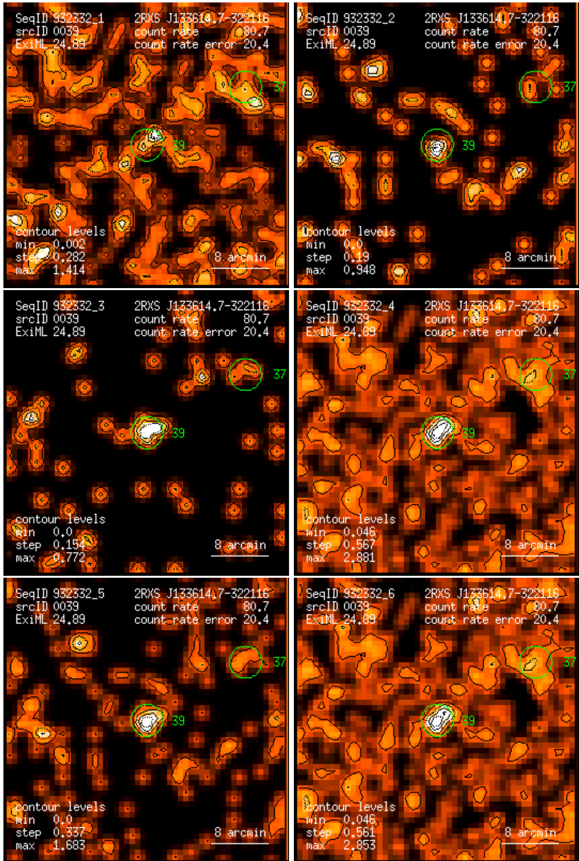
Figure 39: RASS 932332: detection 0039: band rate images, Gaussian filter: (1) PSPC channels 11 – 41, (2) 52 – 90, (3) 91 – 201, (4) 11 – 235, (5) 52 – 201, (6) 11 – 201. Broad band rates in counts/ks. Band rate contour levels in counts/ks/arcmin 2 .
