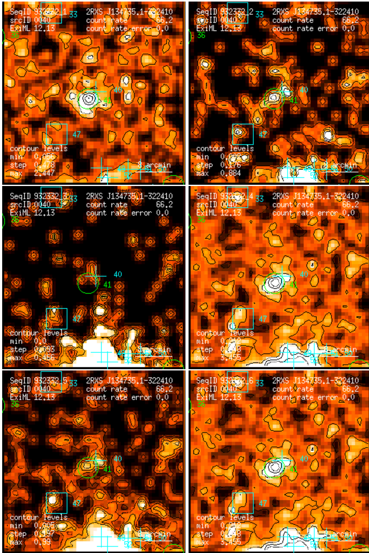
Figure 40: RASS 932332: detection 0040: band rate images, Gaussian filter: (1) PSPC channels 11 – 41, (2) 52 – 90, (3) 91 – 201, (4) 11 – 235, (5) 52 – 201, (6) 11 – 201. Broad band rates in counts/ks. Band rate contour levels in counts/ks/arcmin 2 .
