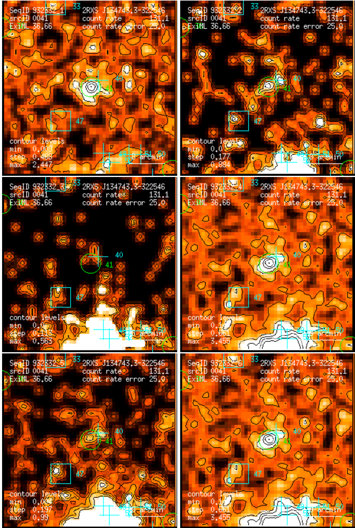
Figure 41: RASS 932332: detection 0041: band rate images, Gaussian filter: (1) PSPC channels 11 – 41, (2) 52 – 90, (3) 91 – 201, (4) 11 – 235, (5) 52 – 201, (6) 11 – 201. Broad band rates in counts/ks. Band rate contour levels in counts/ks/arcmin 2 .
