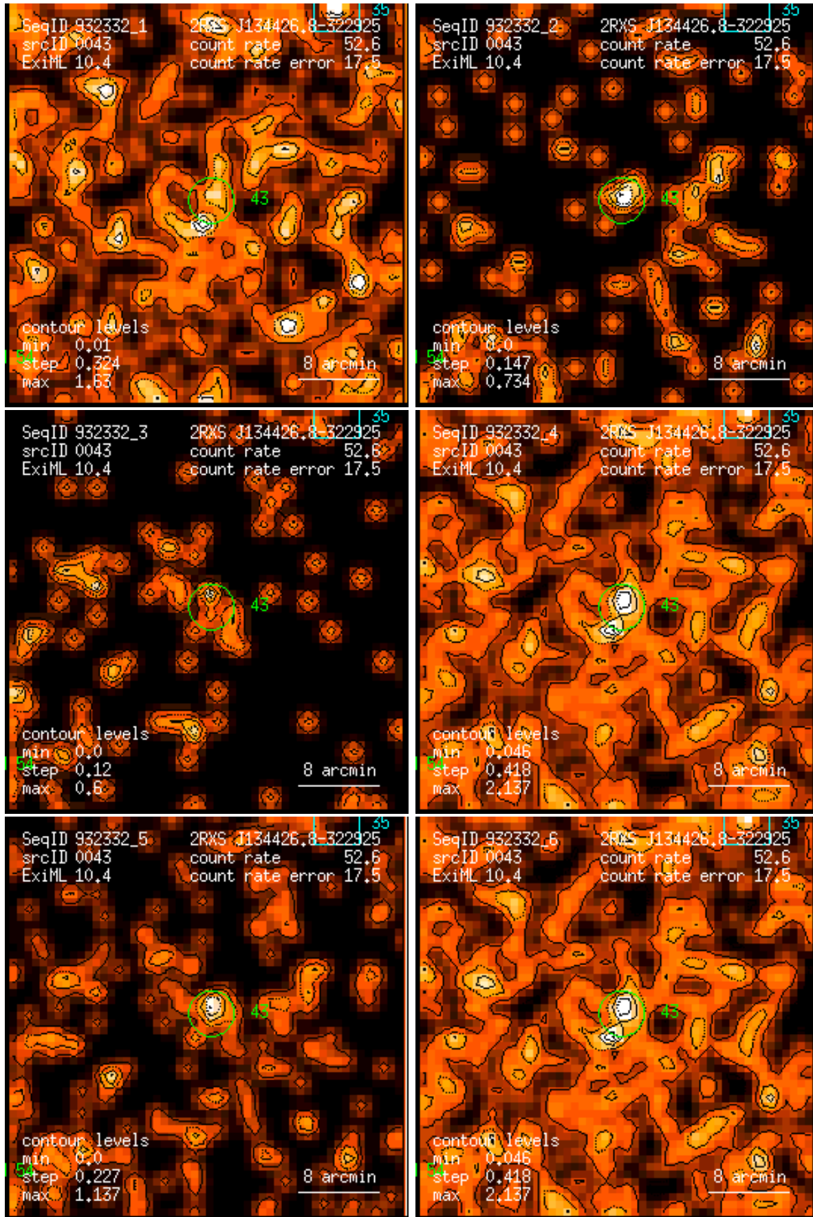
Figure 43: RASS 932332: detection 0043: band rate images, Gaussian filter: (1) PSPC channels 11 – 41, (2) 52 – 90, (3) 91 – 201, (4) 11 – 235, (5) 52 – 201, (6) 11 – 201. Broad band rates in counts/ks. Band rate contour levels in counts/ks/arcmin 2 .
