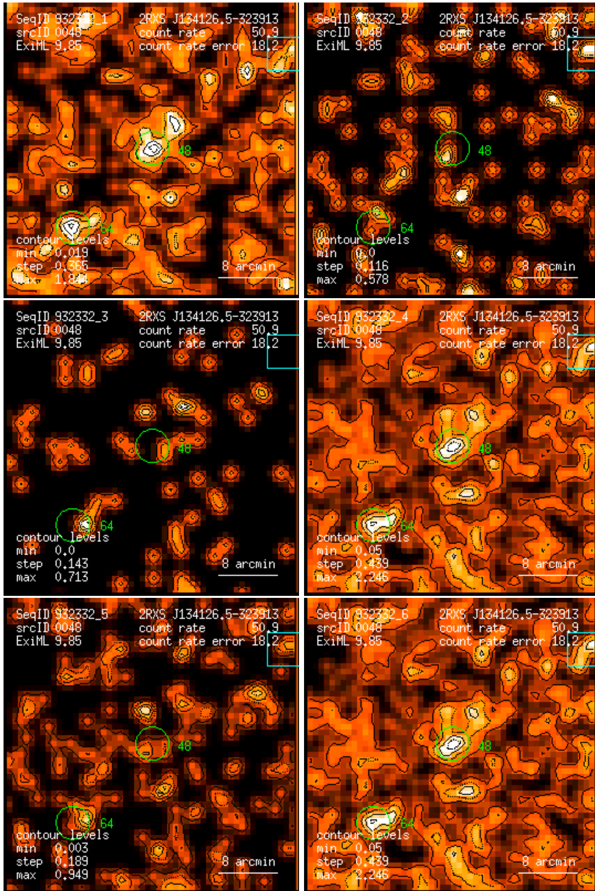
Figure 48: RASS 932332: detection 0048: band rate images, Gaussian filter: (1) PSPC channels 11 – 41, (2) 52 – 90, (3) 91 – 201, (4) 11 – 235, (5) 52 – 201, (6) 11 – 201. Broad band rates in counts/ks. Band rate contour levels in counts/ks/arcmin 2 .
