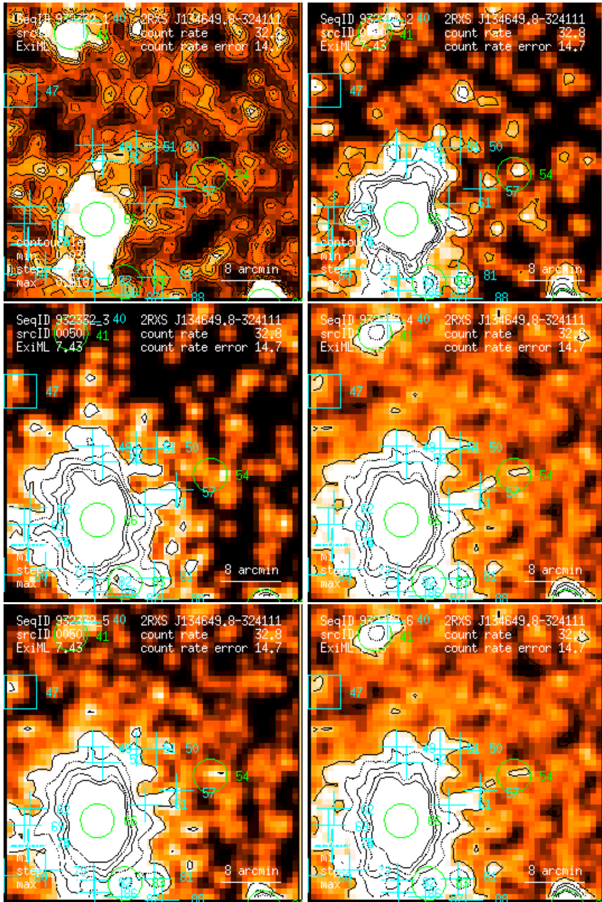
Figure 50: RASS 932332: detection 0050: band rate images, Gaussian filter: (1) PSPC channels 11 – 41, (2) 52 – 90, (3) 91 – 201, (4) 11 – 235, (5) 52 – 201, (6) 11 – 201. Broad band rates in counts/ks. Band rate contour levels in counts/ks/arcmin 2 .
