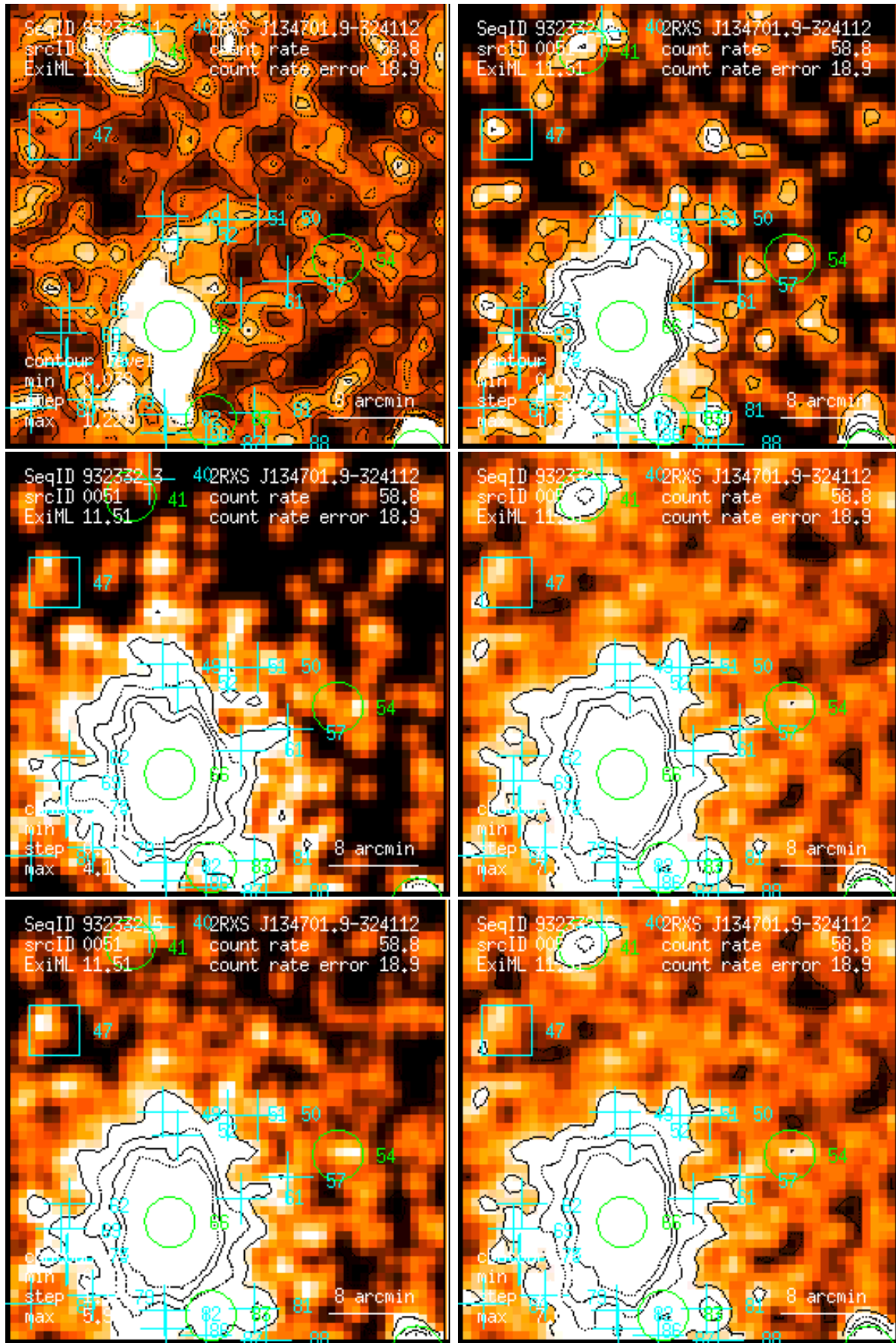
Figure 51: RASS 932332: detection 0051: band rate images, Gaussian filter: (1) PSPC channels 11 – 41, (2) 52 – 90, (3) 91 – 201, (4) 11 – 235, (5) 52 – 201, (6) 11 – 201. Broad band rates in counts/ks. Band rate contour levels in counts/ks/arcmin 2 .
