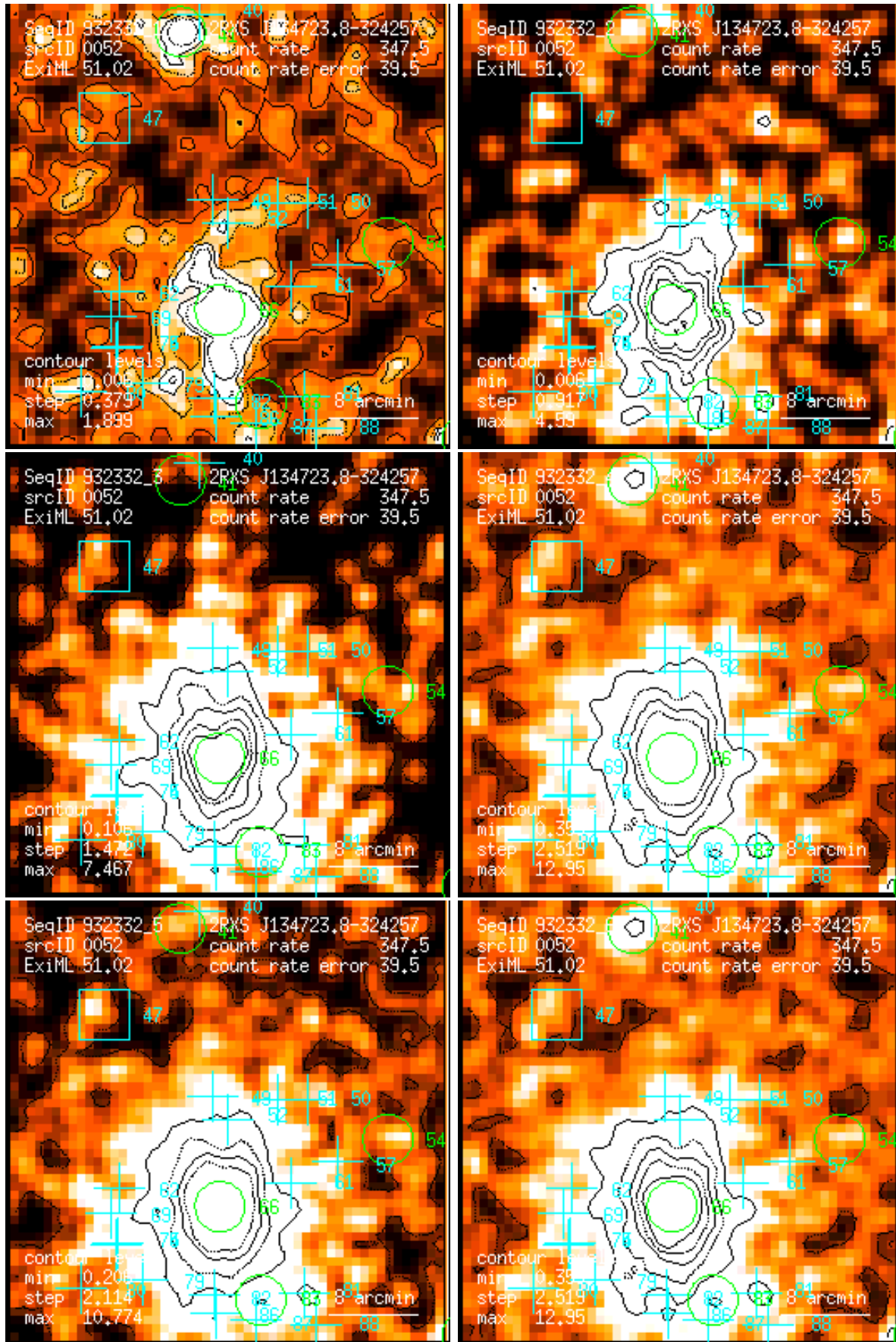
Figure 52: RASS 932332: detection 0052: band rate images, Gaussian filter: (1) PSPC channels 11 – 41, (2) 52 – 90, (3) 91 – 201, (4) 11 – 235, (5) 52 – 201, (6) 11 – 201. Broad band rates in counts/ks. Band rate contour levels in counts/ks/arcmin 2 .
