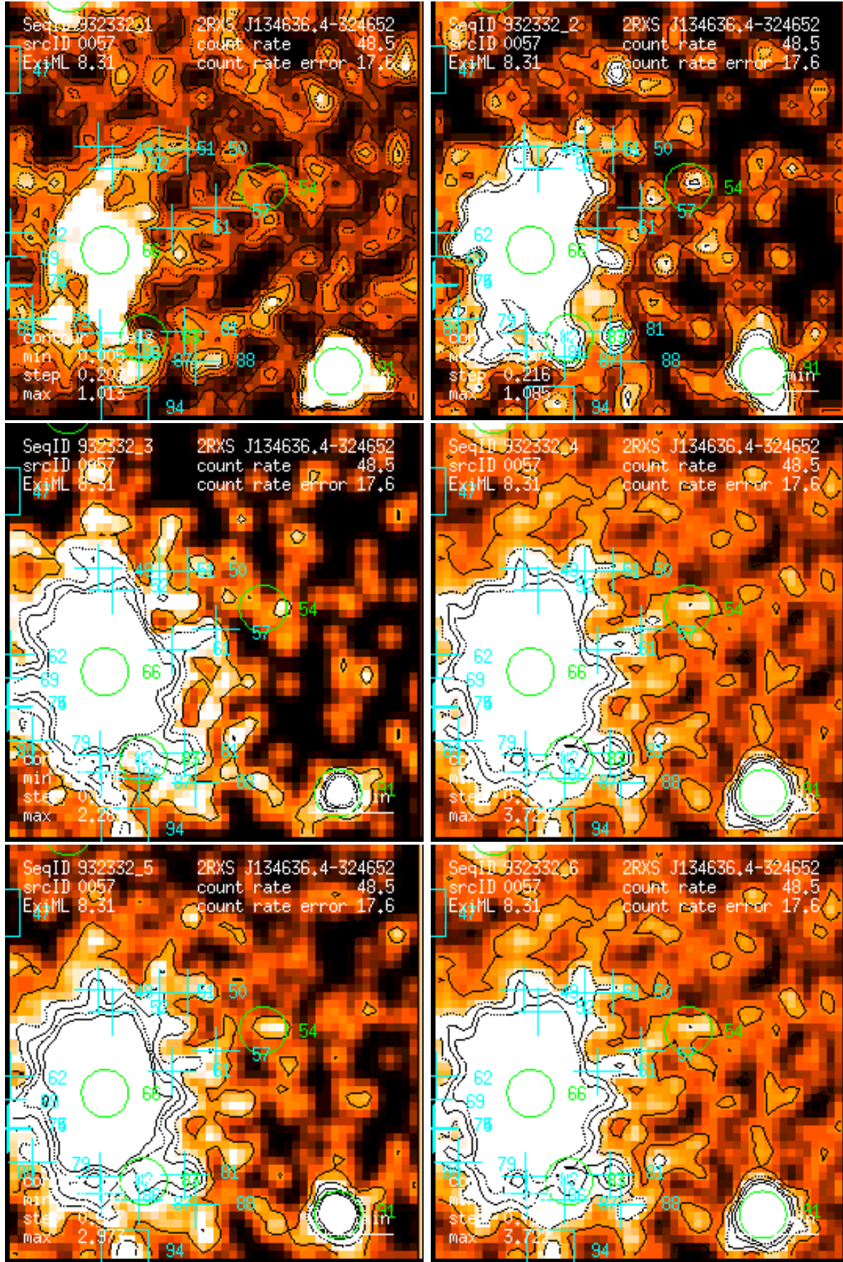
Figure 57: RASS 932332: detection 0057: band rate images, Gaussian filter: (1) PSPC channels 11 – 41, (2) 52 – 90, (3) 91 – 201, (4) 11 – 235, (5) 52 – 201, (6) 11 – 201. Broad band rates in counts/ks. Band rate contour levels in counts/ks/arcmin 2 .
