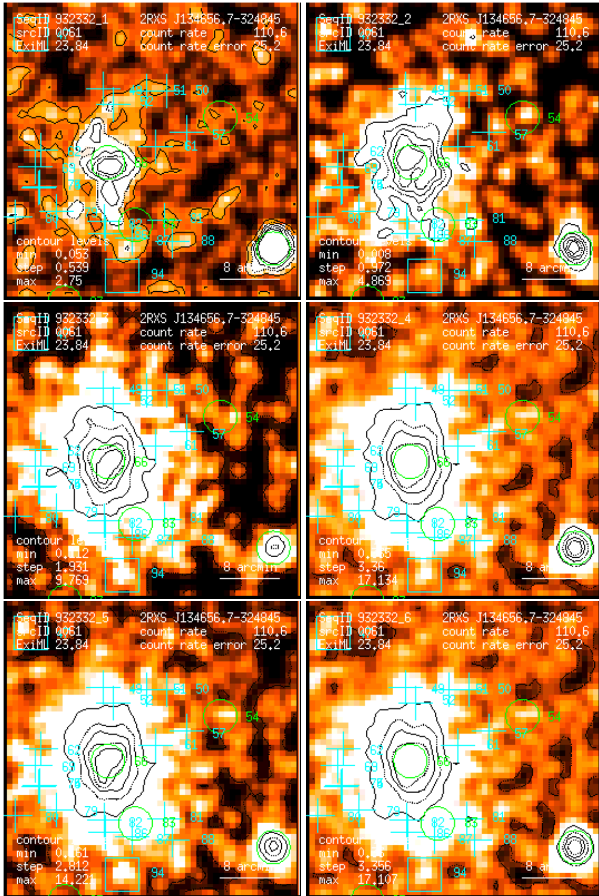
Figure 61: RASS 932332: detection 0061: band rate images, Gaussian filter: (1) PSPC channels 11 – 41, (2) 52 – 90, (3) 91 – 201, (4) 11 – 235, (5) 52 – 201, (6) 11 – 201. Broad band rates in counts/ks. Band rate contour levels in counts/ks/arcmin 2 .
