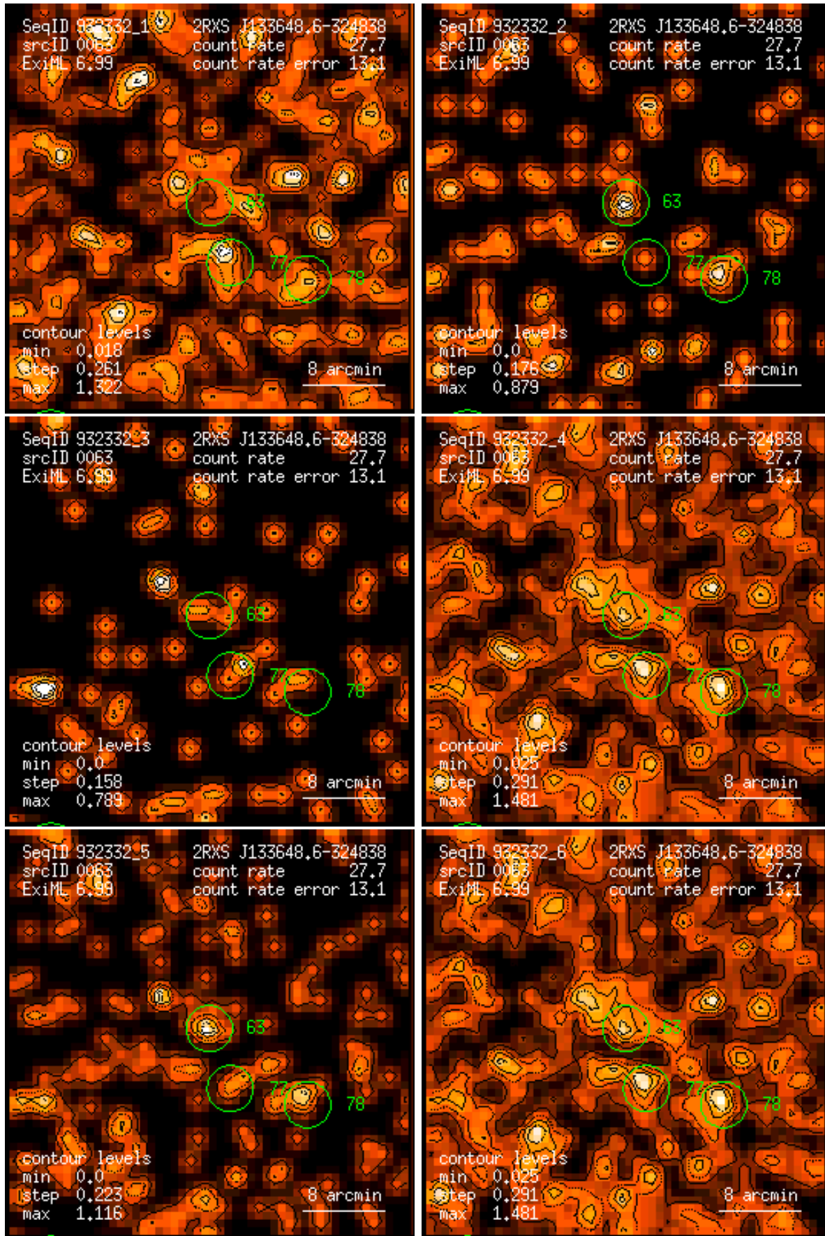
Figure 63: RASS 932332: detection 0063: band rate images, Gaussian filter: (1) PSPC channels 11 – 41, (2) 52 – 90, (3) 91 – 201, (4) 11 – 235, (5) 52 – 201, (6) 11 – 201. Broad band rates in counts/ks. Band rate contour levels in counts/ks/arcmin 2 .
