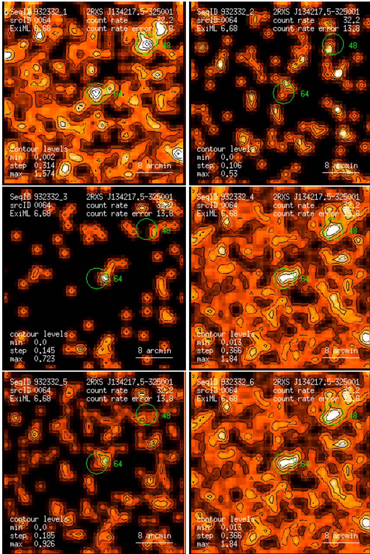
Figure 64: RASS 932332: detection 0064: band rate images, Gaussian filter: (1) PSPC channels 11 – 41, (2) 52 – 90, (3) 91 – 201, (4) 11 – 235, (5) 52 – 201, (6) 11 – 201. Broad band rates in counts/ks. Band rate contour levels in counts/ks/arcmin 2 .
