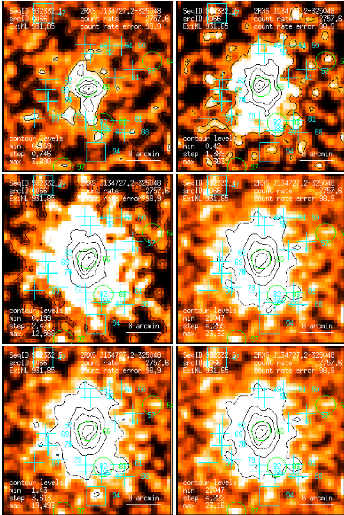
Figure 66: RASS 932332: detection 0066: band rate images, Gaussian filter: (1) PSPC channels 11 – 41, (2) 52 – 90, (3) 91 – 201, (4) 11 – 235, (5) 52 – 201, (6) 11 – 201. Broad band rates in counts/ks. Band rate contour levels in counts/ks/arcmin 2 .
