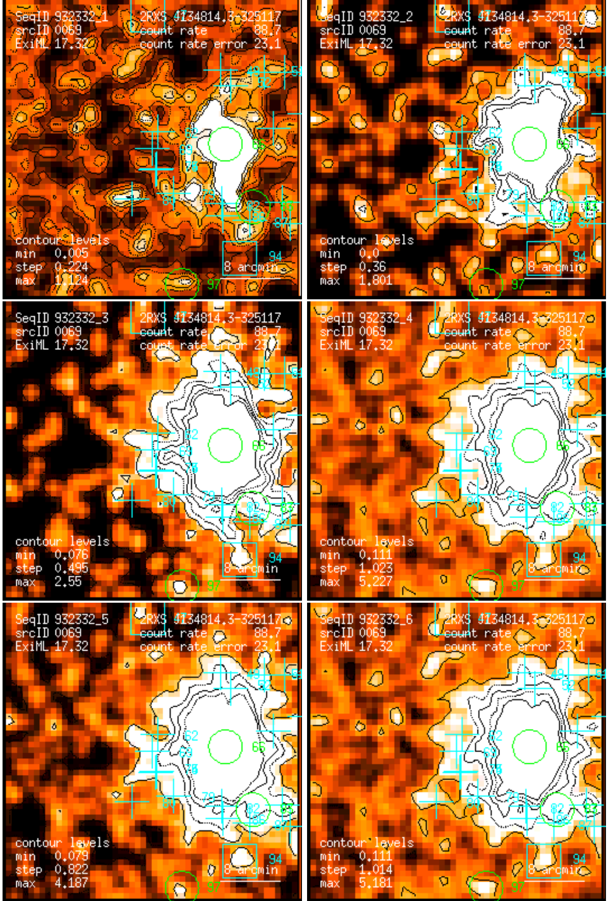
Figure 69: RASS 932332: detection 0069: band rate images, Gaussian filter: (1) PSPC channels 11 – 41, (2) 52 – 90, (3) 91 – 201, (4) 11 – 235, (5) 52 – 201, (6) 11 – 201. Broad band rates in counts/ks. Band rate contour levels in counts/ks/arcmin 2 .
