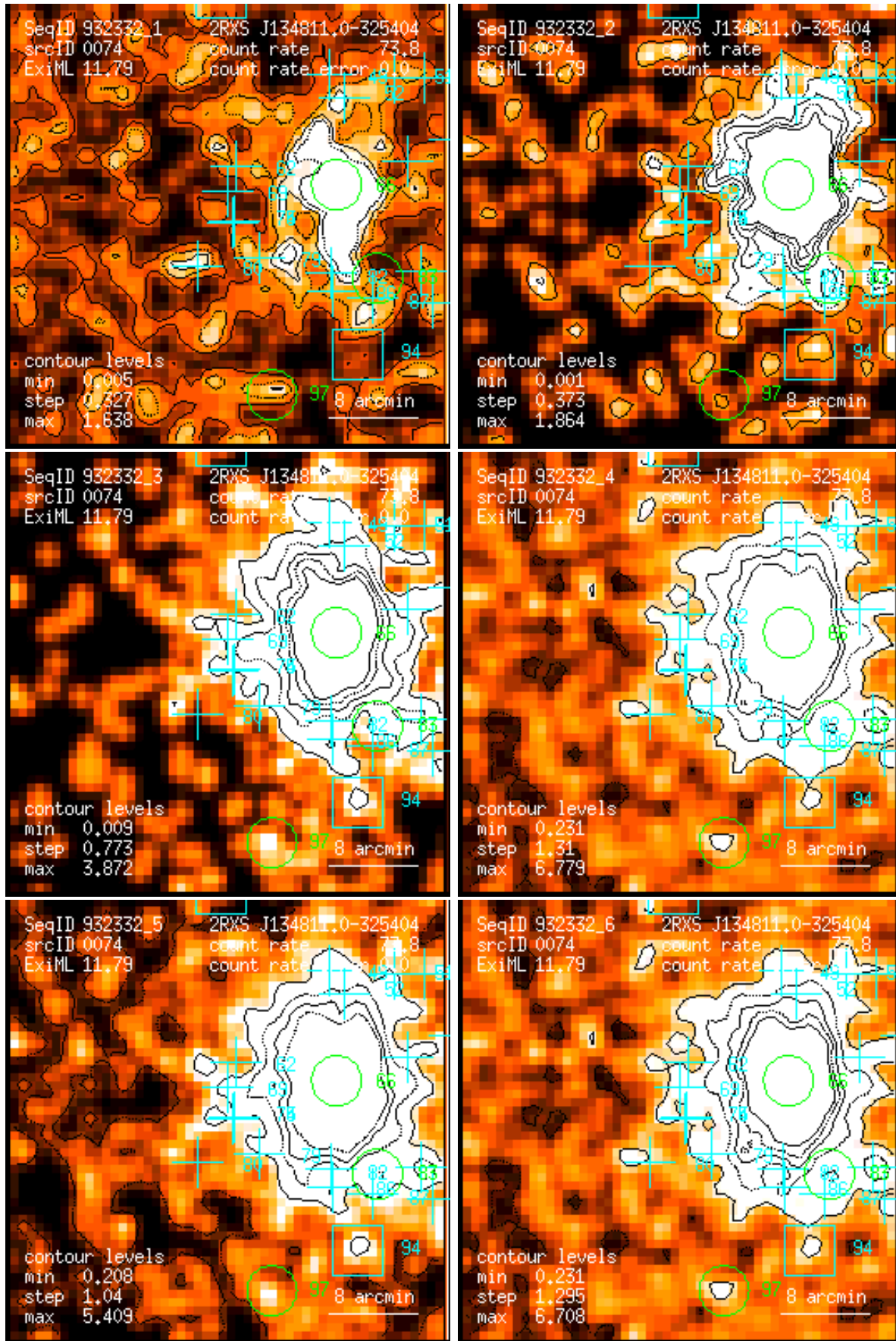
Figure 74: RASS 932332: detection 0074: band rate images, Gaussian filter: (1) PSPC channels 11 – 41, (2) 52 – 90, (3) 91 – 201, (4) 11 – 235, (5) 52 – 201, (6) 11 – 201. Broad band rates in counts/ks. Band rate contour levels in counts/ks/arcmin 2 .
