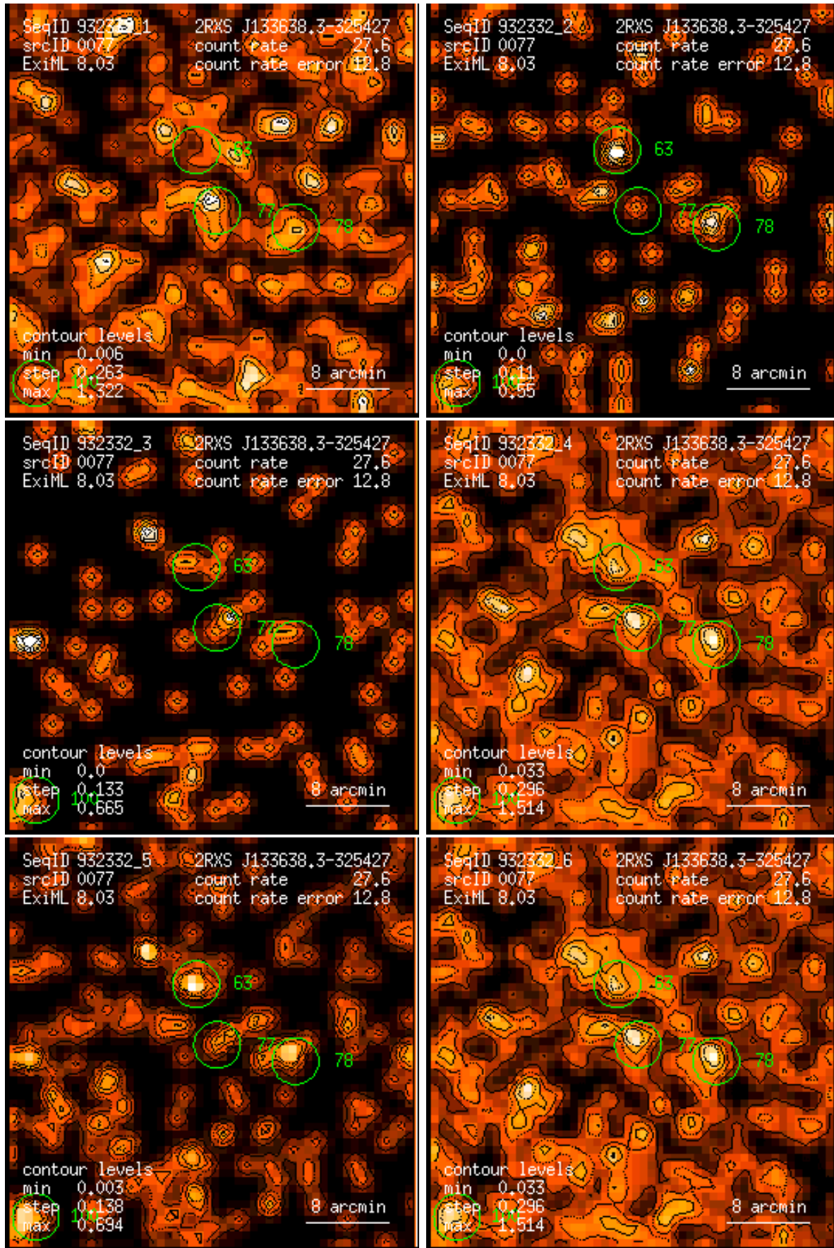
Figure 77: RASS 932332: detection 0077: band rate images, Gaussian filter: (1) PSPC channels 11 – 41, (2) 52 – 90, (3) 91 – 201, (4) 11 – 235, (5) 52 – 201, (6) 11 – 201. Broad band rates in counts/ks. Band rate contour levels in counts/ks/arcmin 2 .
