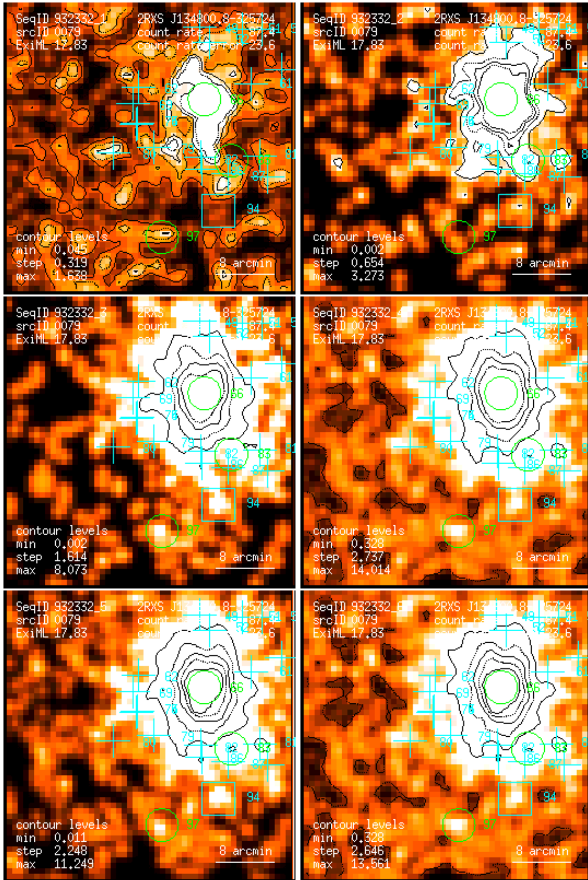
Figure 79: RASS 932332: detection 0079: band rate images, Gaussian filter: (1) PSPC channels 11 – 41, (2) 52 – 90, (3) 91 – 201, (4) 11 – 235, (5) 52 – 201, (6) 11 – 201. Broad band rates in counts/ks. Band rate contour levels in counts/ks/arcmin 2 .
