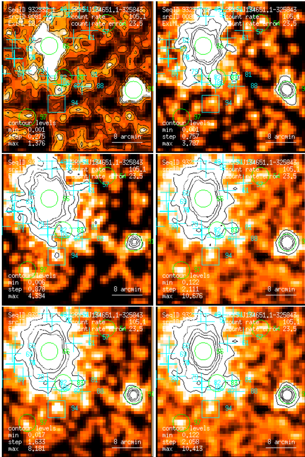
Figure 81: RASS 932332: detection 0081: band rate images, Gaussian filter: (1) PSPC channels 11 – 41, (2) 52 – 90, (3) 91 – 201, (4) 11 – 235, (5) 52 – 201, (6) 11 – 201. Broad band rates in counts/ks. Band rate contour levels in counts/ks/arcmin 2 .
