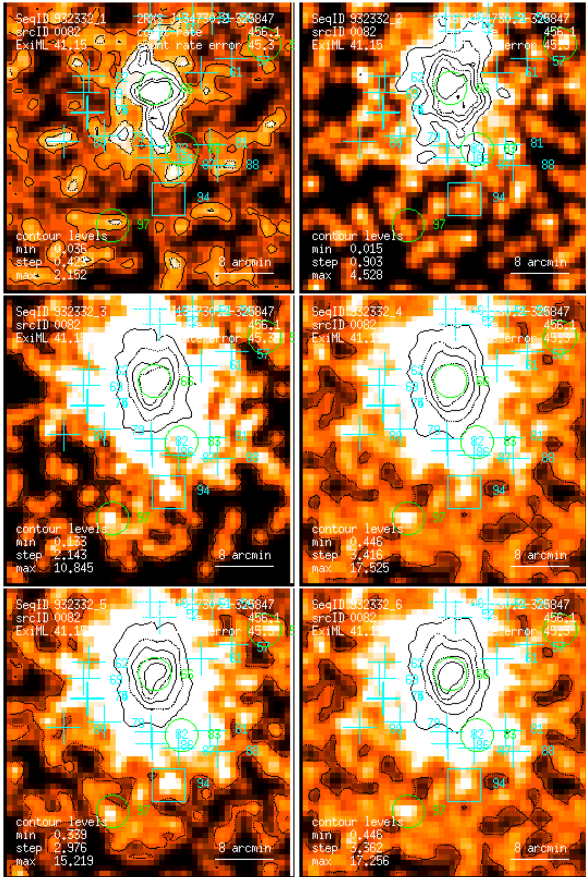
Figure 82: RASS 932332: detection 0082: band rate images, Gaussian filter: (1) PSPC channels 11 – 41, (2) 52 – 90, (3) 91 – 201, (4) 11 – 235, (5) 52 – 201, (6) 11 – 201. Broad band rates in counts/ks. Band rate contour levels in counts/ks/arcmin 2 .
