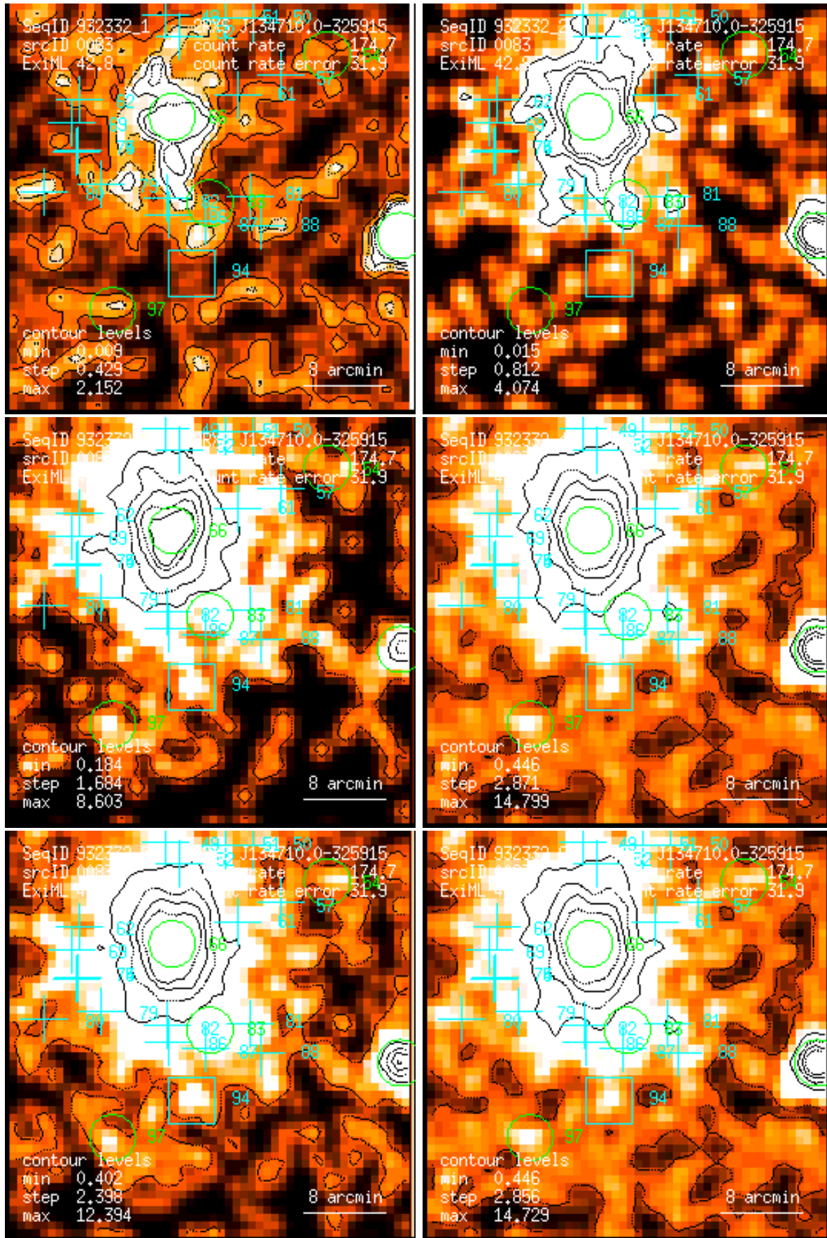
Figure 83: RASS 932332: detection 0083: band rate images, Gaussian filter: (1) PSPC channels 11 – 41, (2) 52 – 90, (3) 91 – 201, (4) 11 – 235, (5) 52 – 201, (6) 11 – 201. Broad band rates in counts/ks. Band rate contour levels in counts/ks/arcmin 2 .
